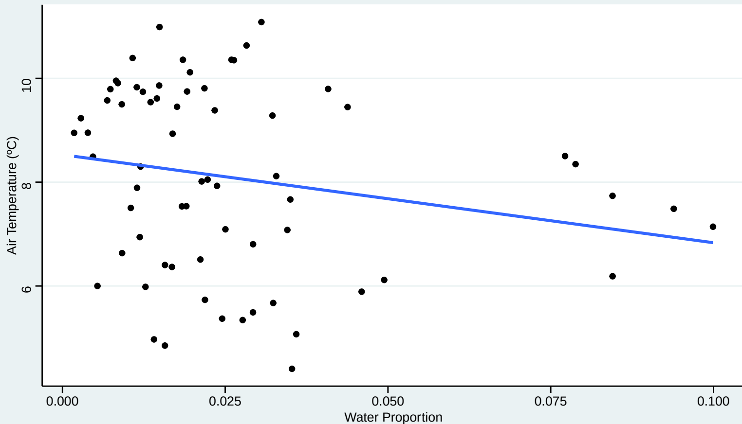
Average 2020 Air Temperature by Michigan County Water Proportion
