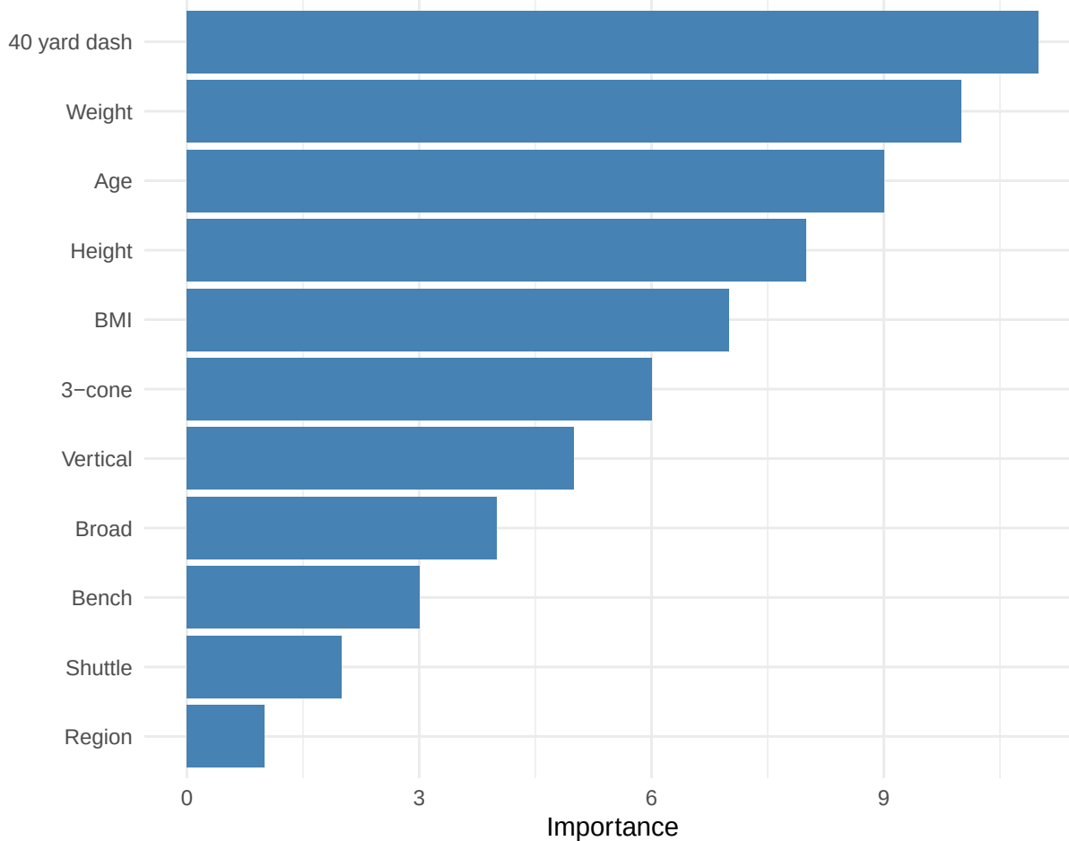
Variable Importance for Top 3-Round Picks
