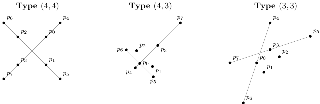
Figure 5: Exact representatives of the three realizable line–circle incidence types at n = 8 and c(P) = 18 . Coordinates are listed in the text; gray segments show all maximal lines, and circles are omitted for legibility.
