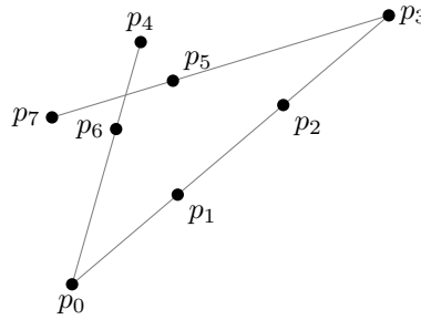
Figure 4: The rational eight-point construction with 17 circles. Gray segments show all maximal collinear subsets; the circles are listed in the text.
