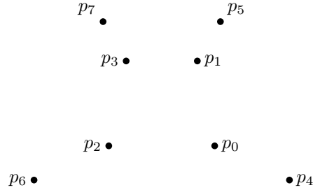
Figure 6: The eight-point construction for the no-three-collinear variant. Only the points are drawn; displaying all twenty circles would obscure the configuration.
