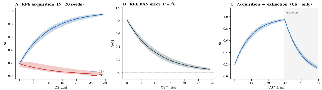
Figure 2. RPE on the connectome substrate. (A) Acquisition curve with N=20 seed variance bands; CS+ m_{\text{hat}} rises while CS- remains flat. (B) DAN error r - m_{\text{hat}} decays to \sim 0.06 by
