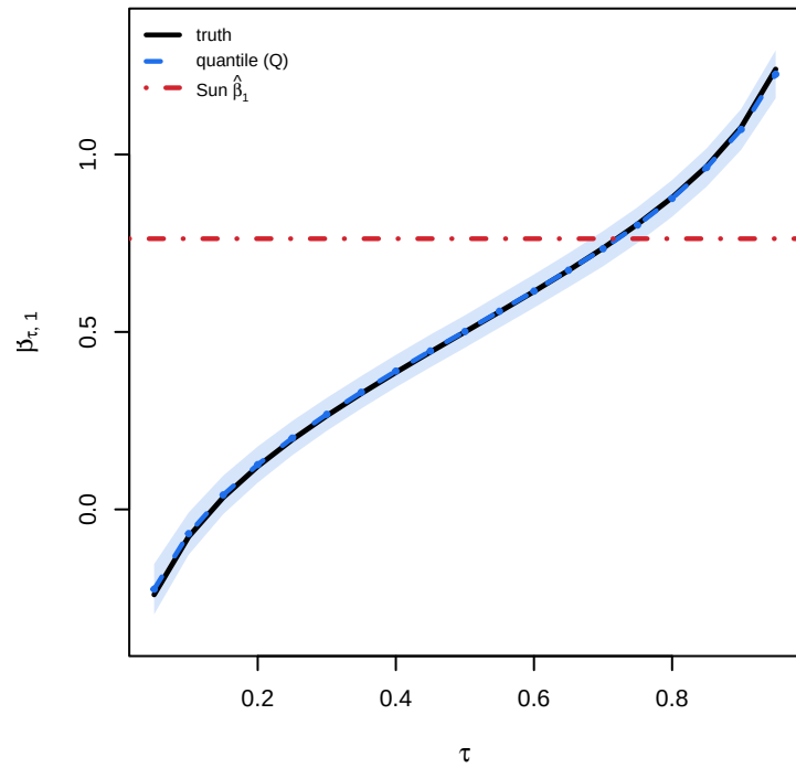
DGP3: non-proportional mean
