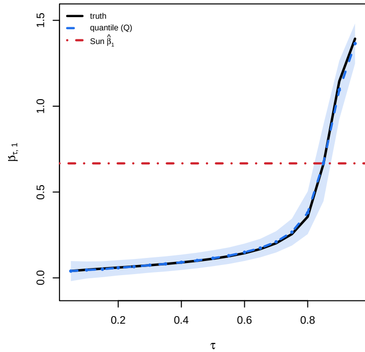
DGP4: tail-specific effect
