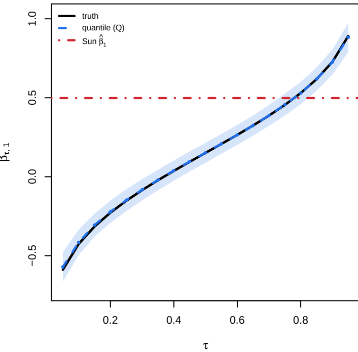
DGP2: dispersion varies
