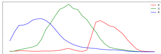
Estimated camera sensor sensitivity
