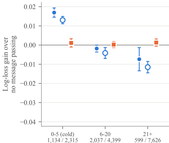
(a) Prior opponents (less-recorded player)
