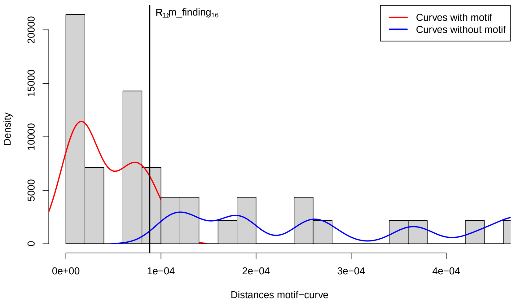
Distances motif-curve – Cluster 16
