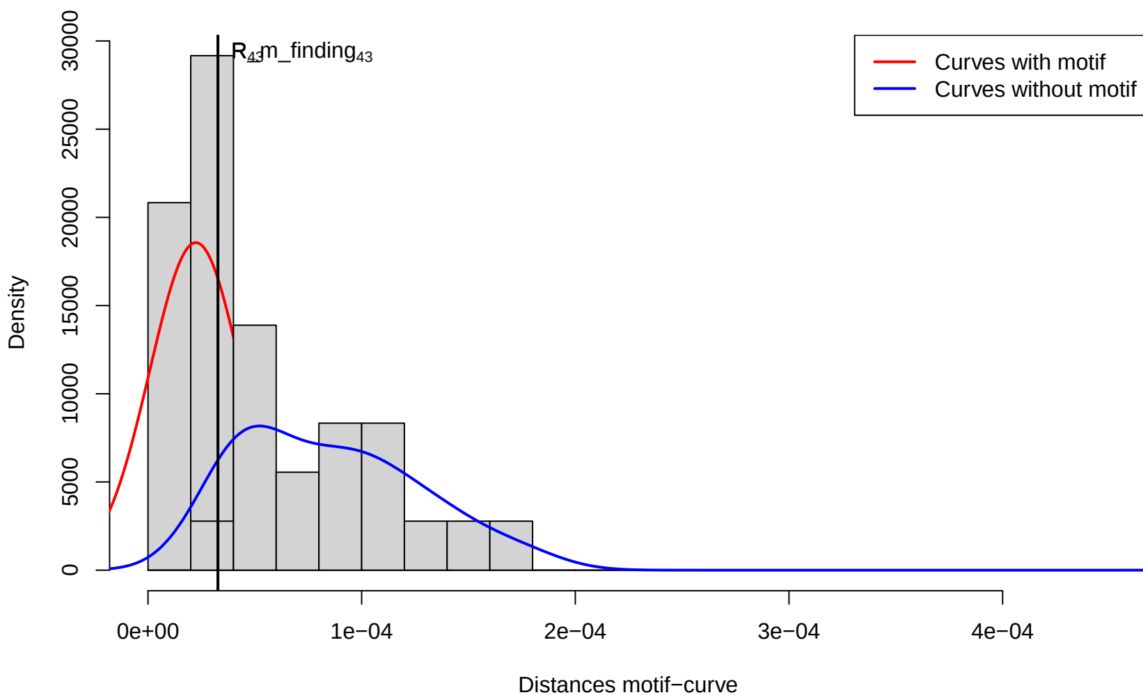
Distances motif-curve – Cluster 43
