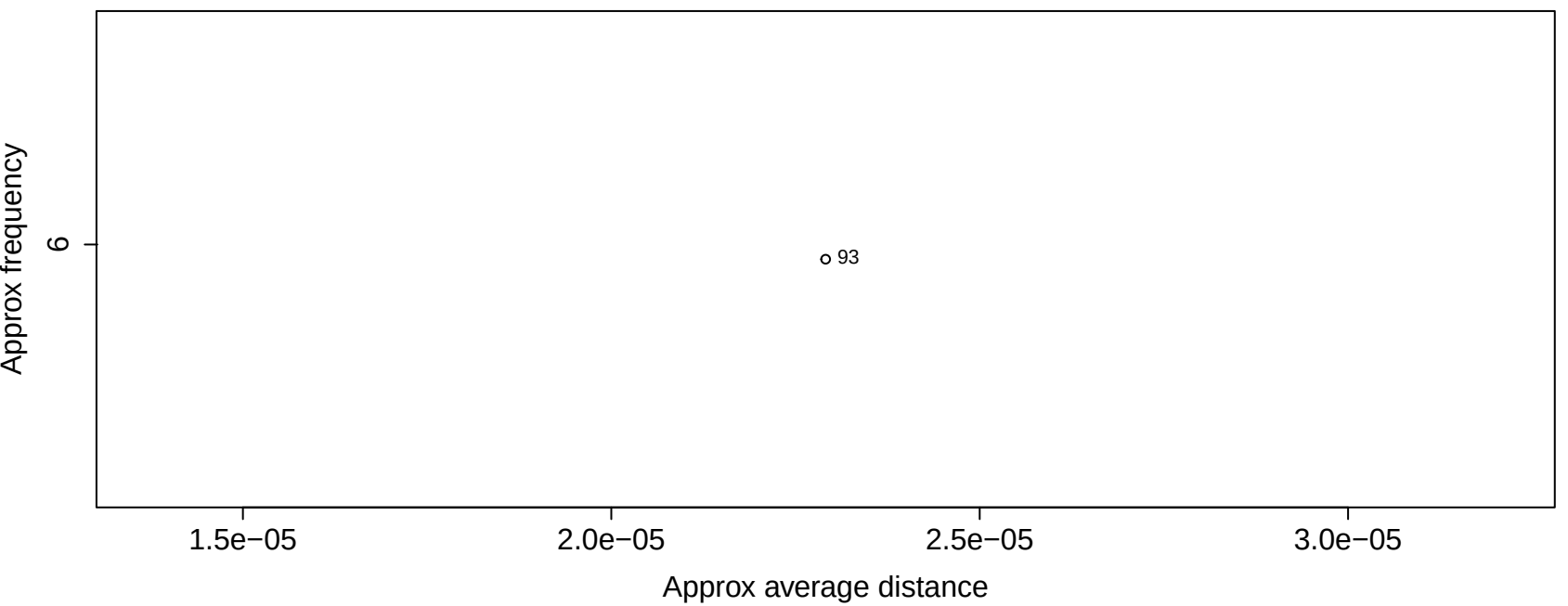
Motif in Cluster 40
