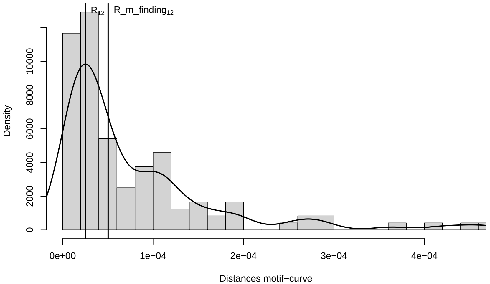
Distances motif-curve – Cluster 12
