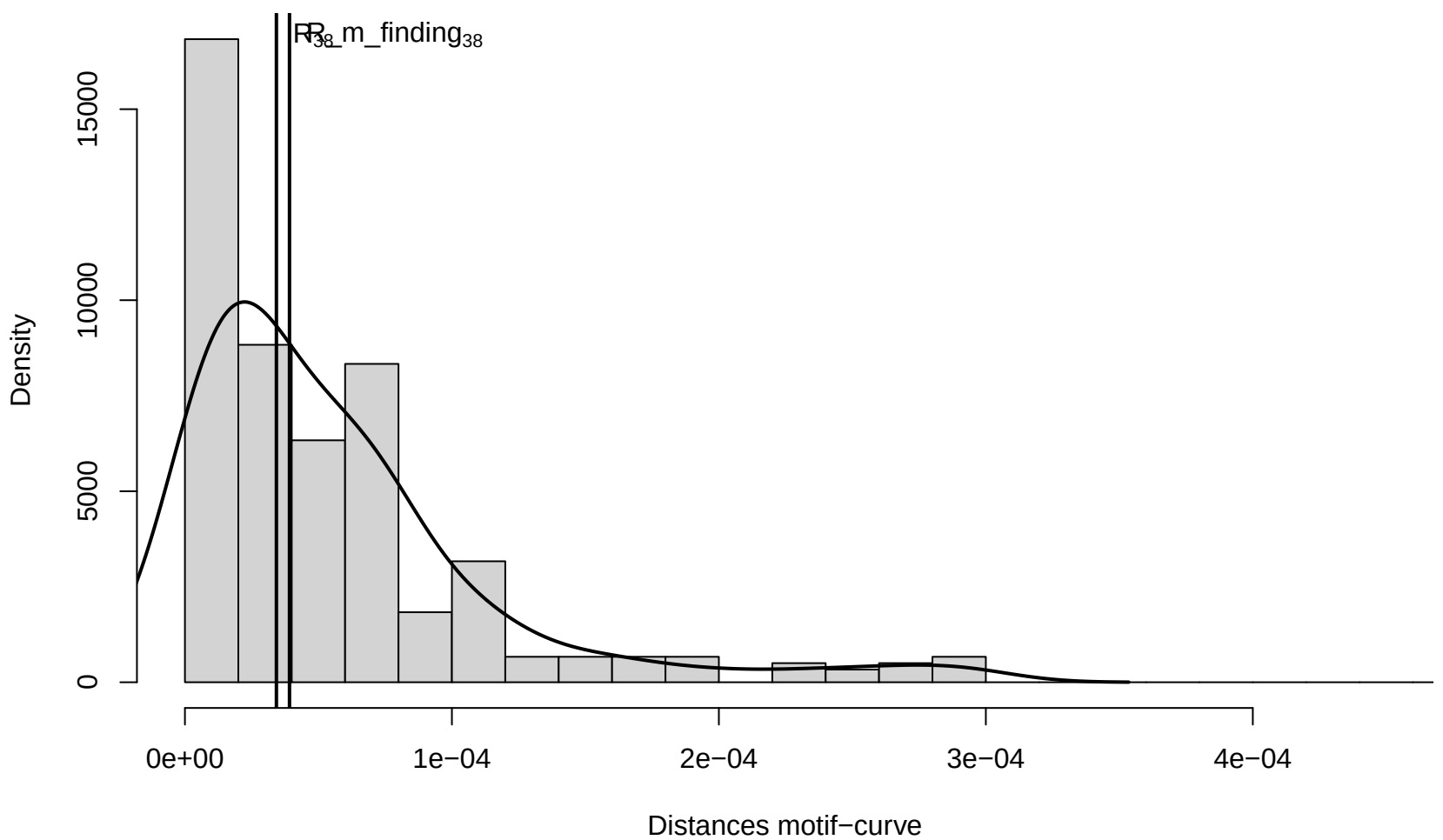
Distances motif-curve – Cluster 38
