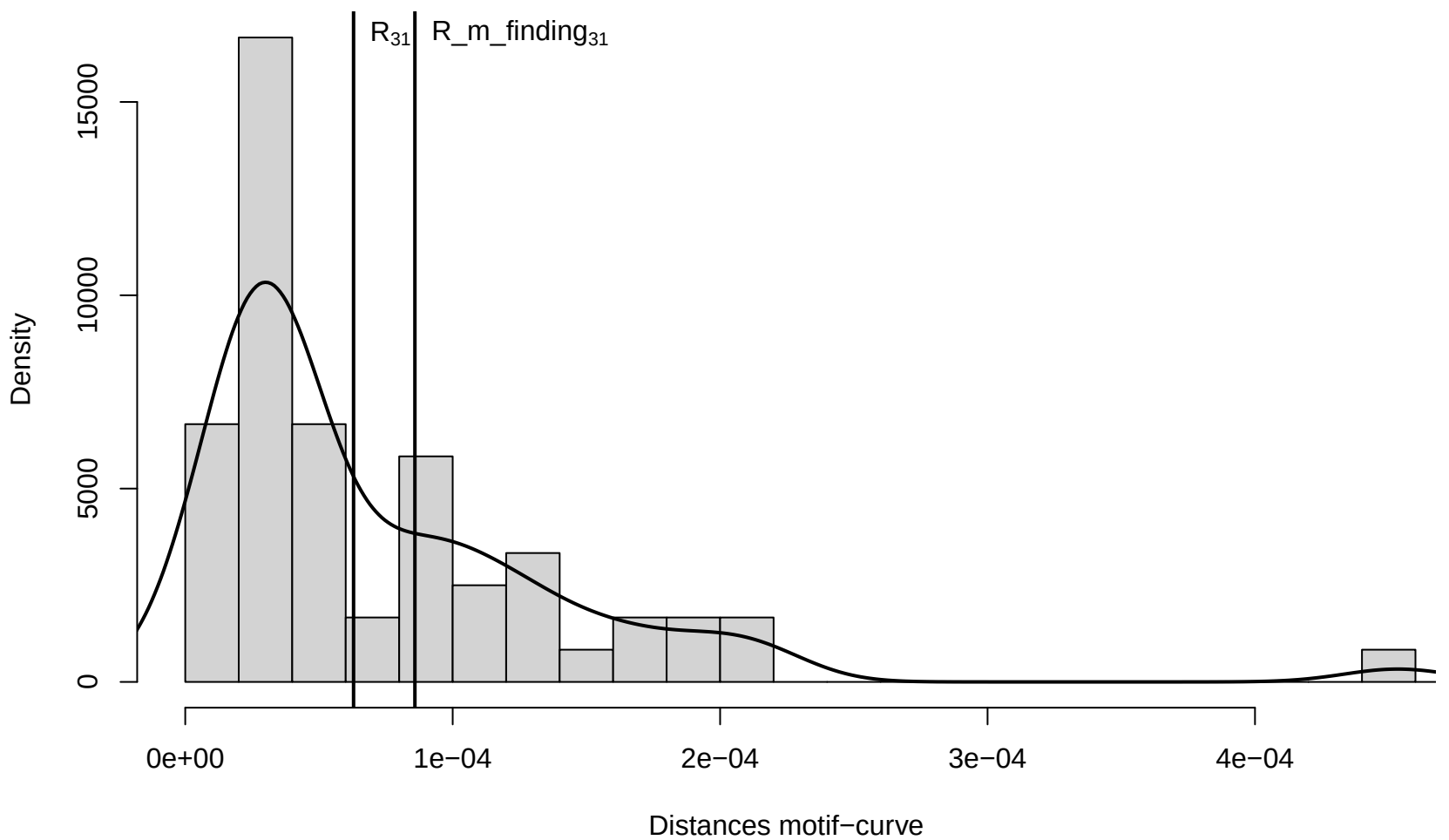
Distances motif-curve – Cluster 31
