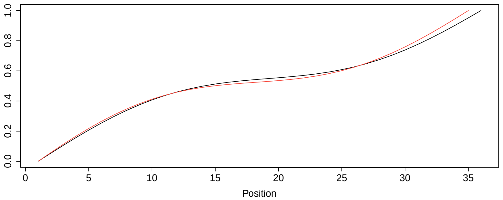
Motifs in Cluster 35
