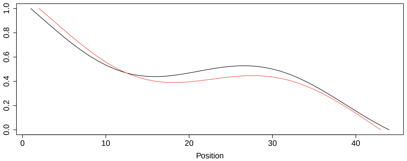
Motifs in Cluster 27
