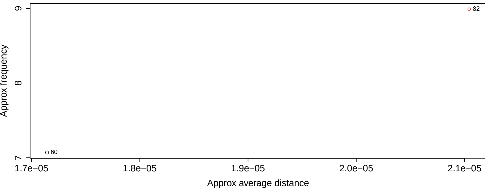
Motif in Cluster 28
