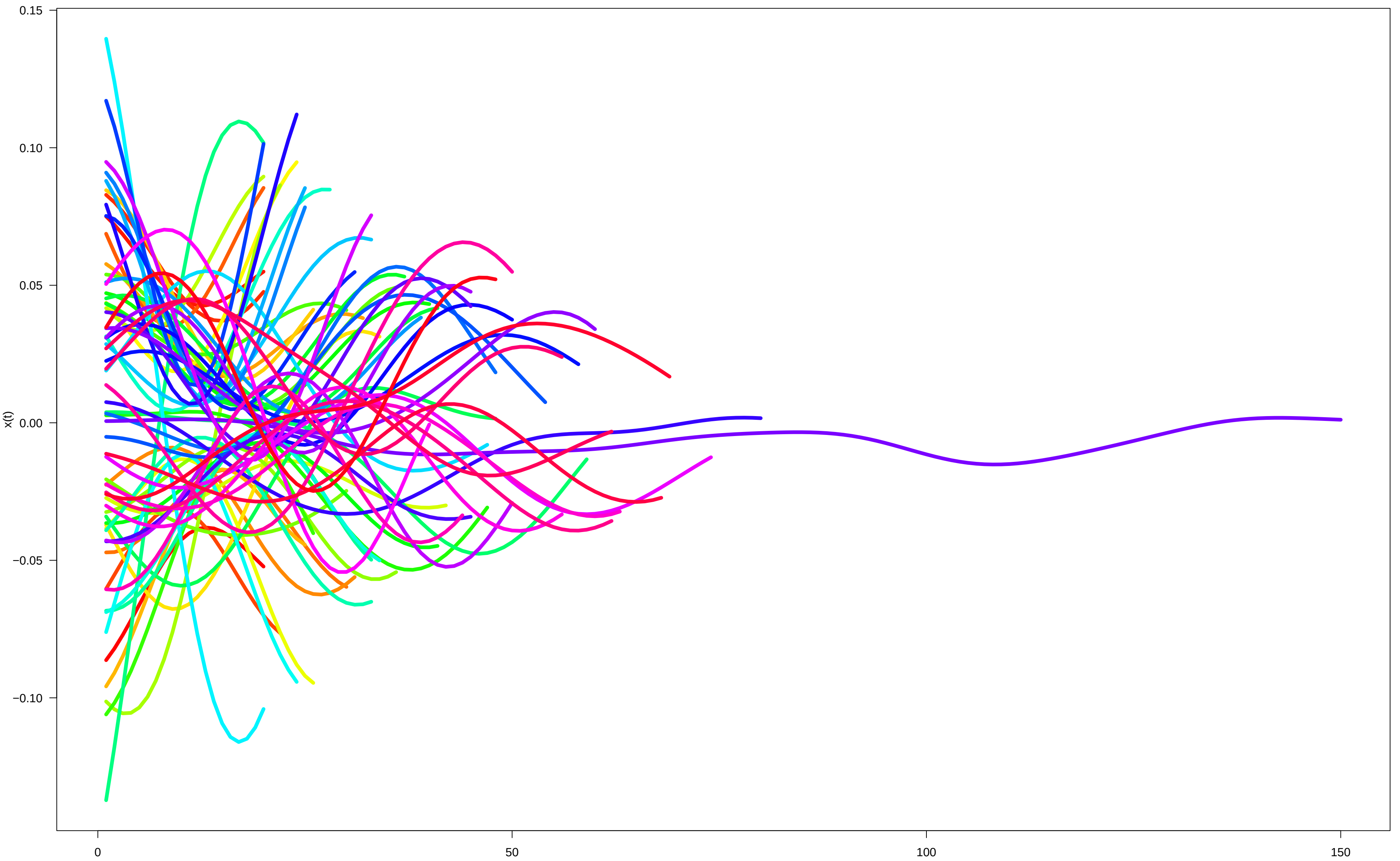
x(t) derivative
