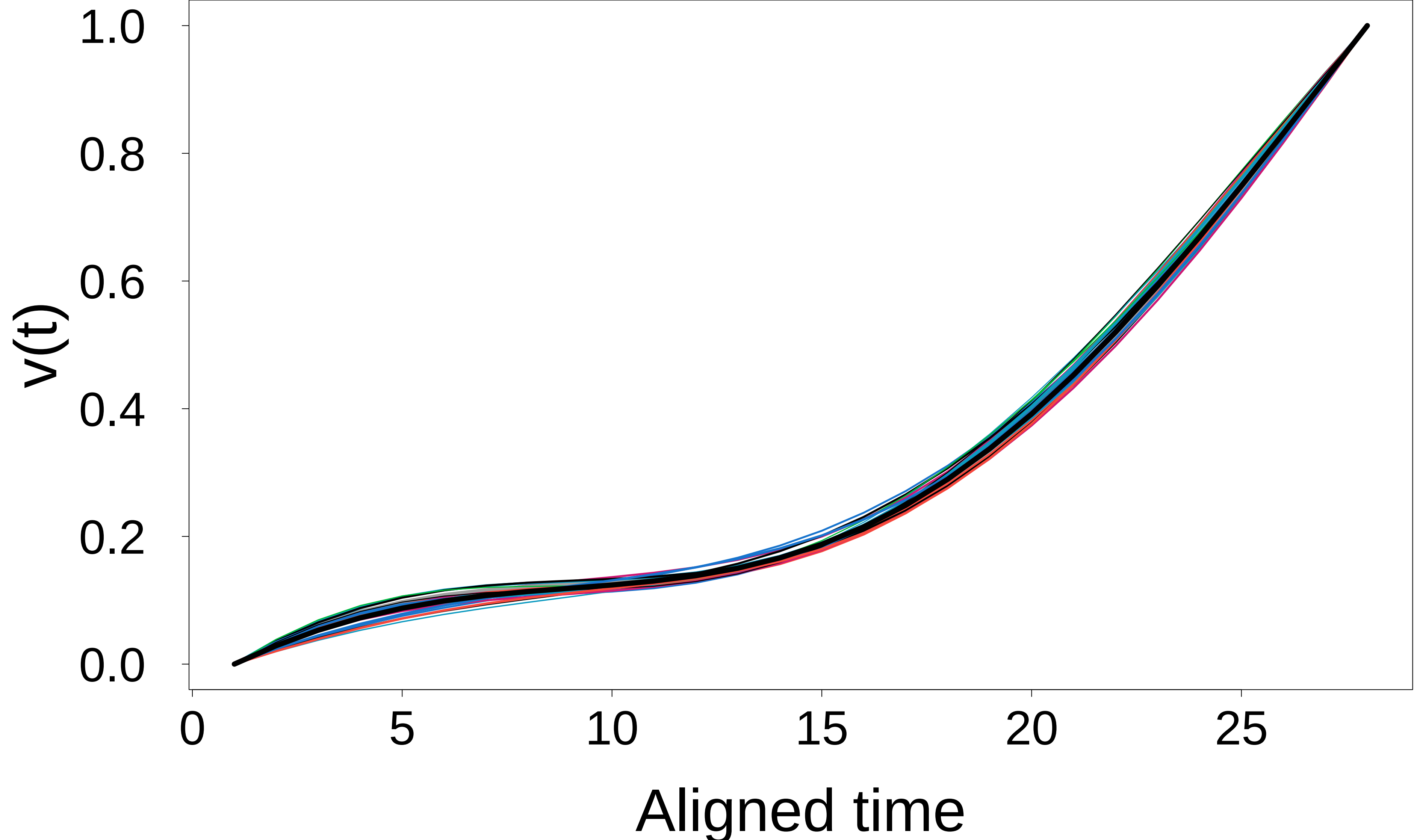
Motif 32 (20 occurrences)
