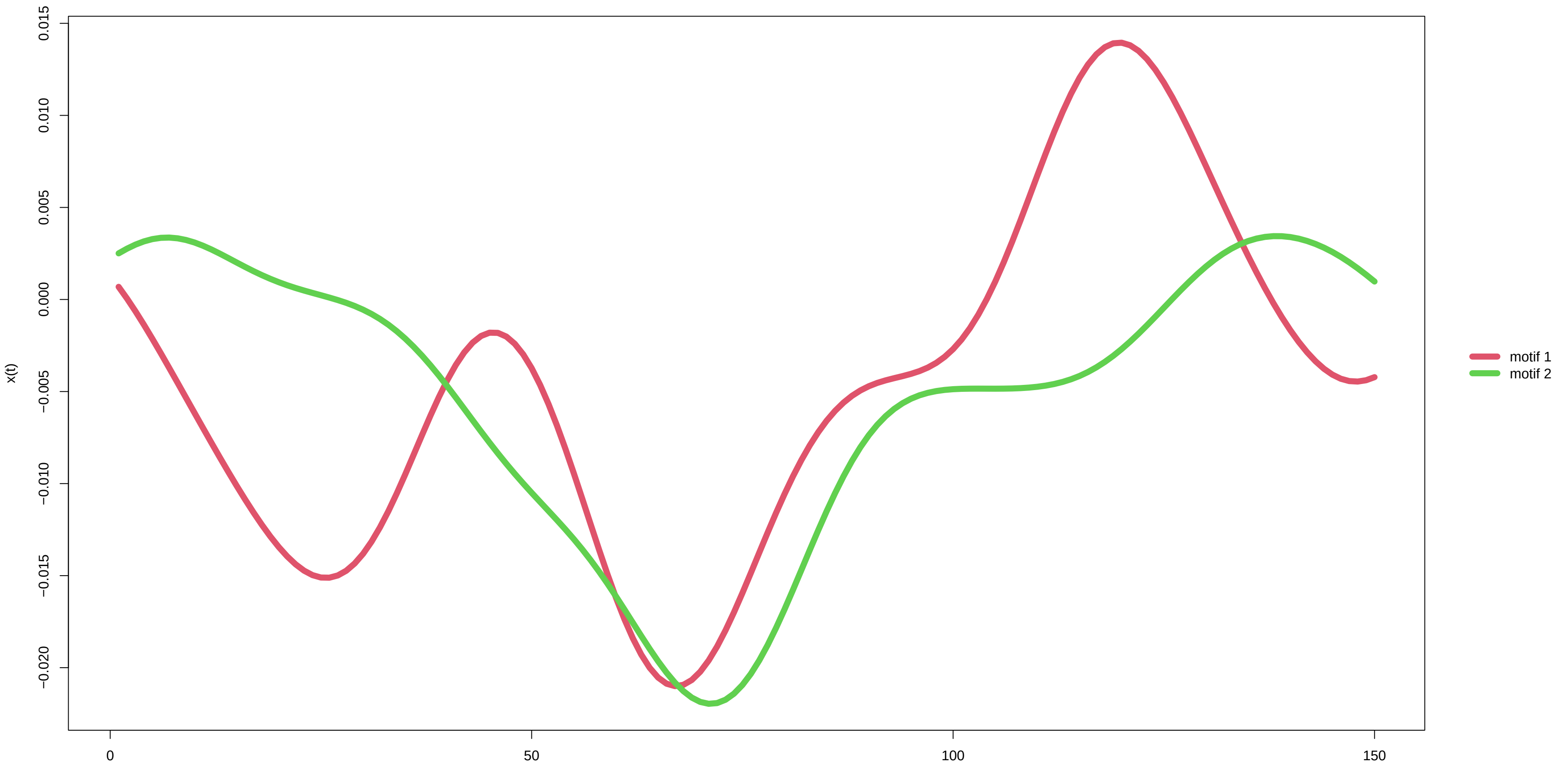
x(t) derivative
