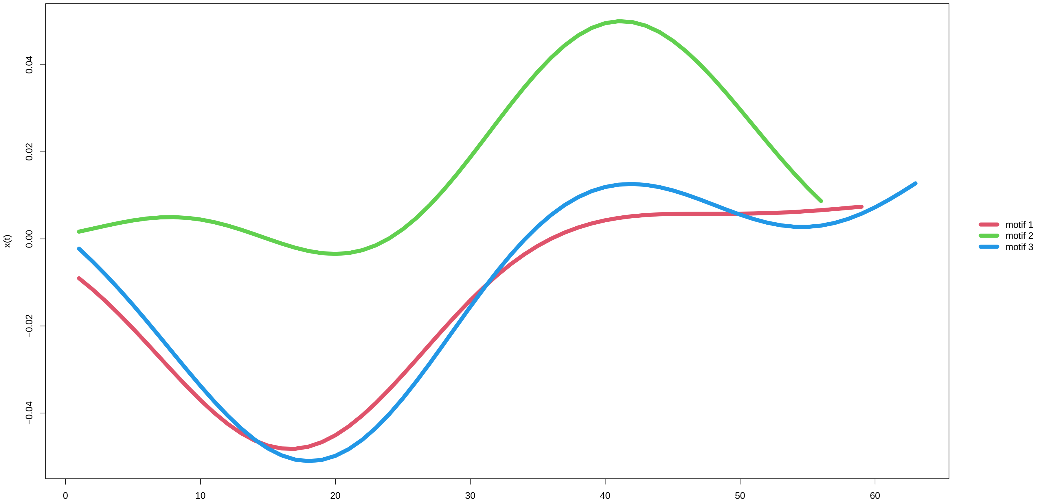
x(t) derivative
