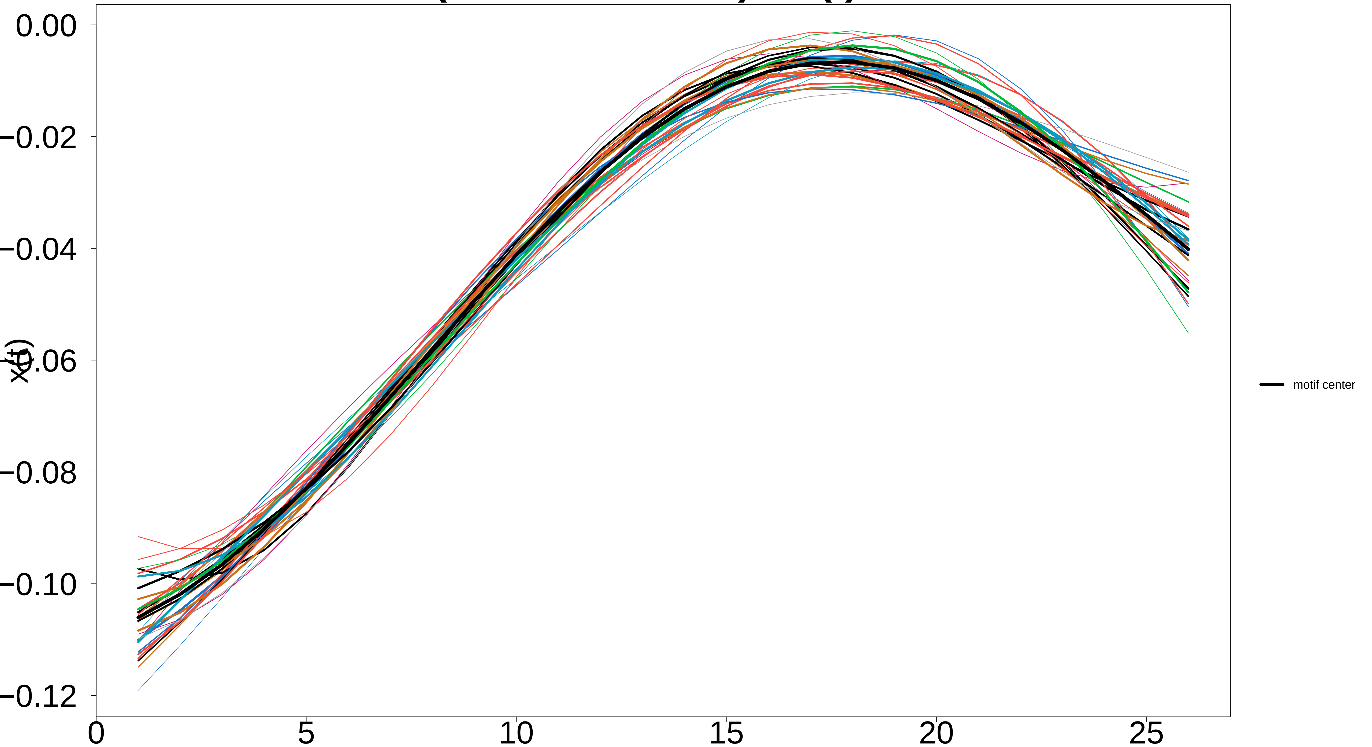
Motif 21 (31 occurrences) – x(t) derivative
