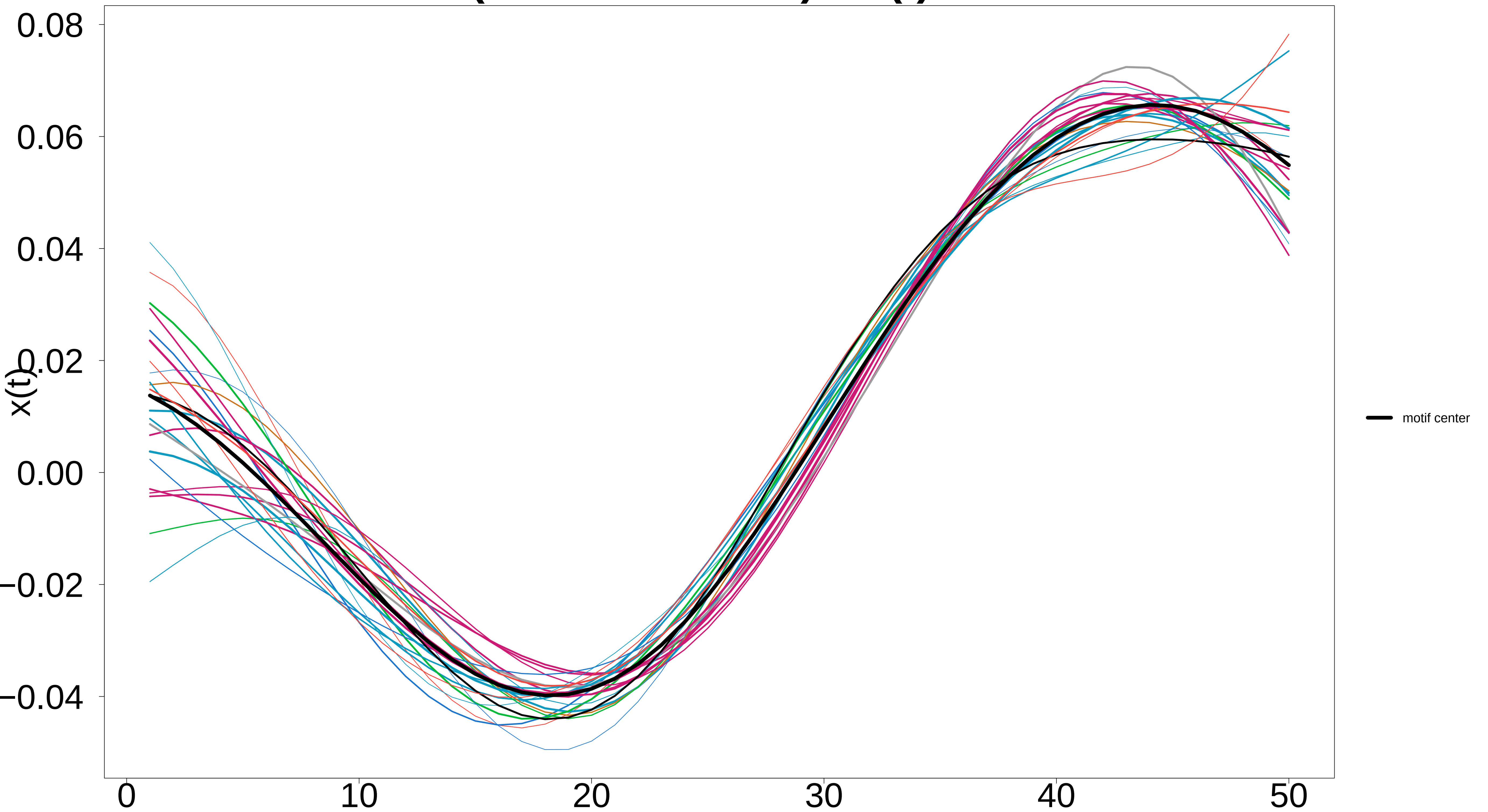
Motif 61 (23 occurrences) – x(t) derivative
