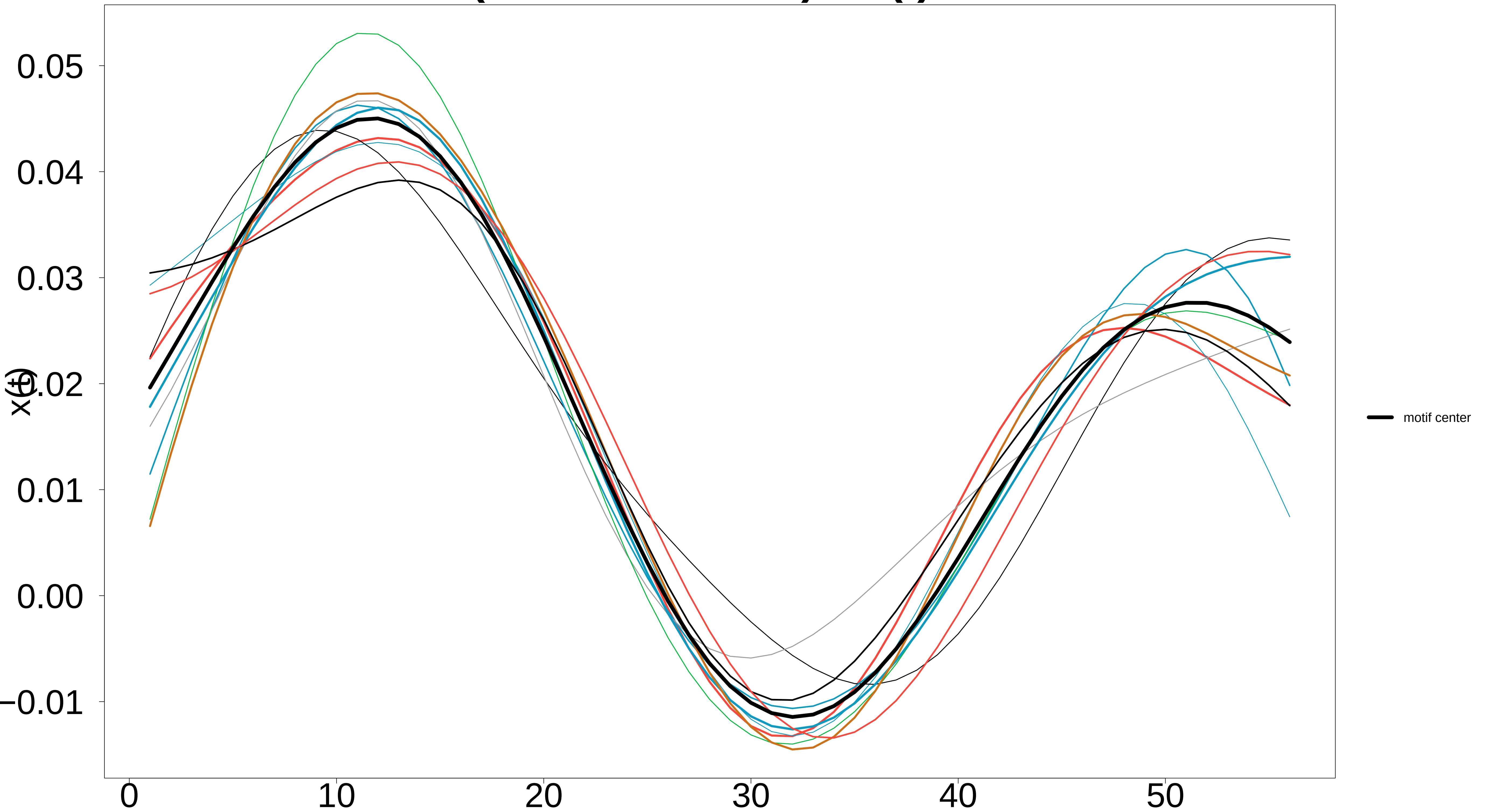
Motif 63 (10 occurrences) – x(t) derivative
