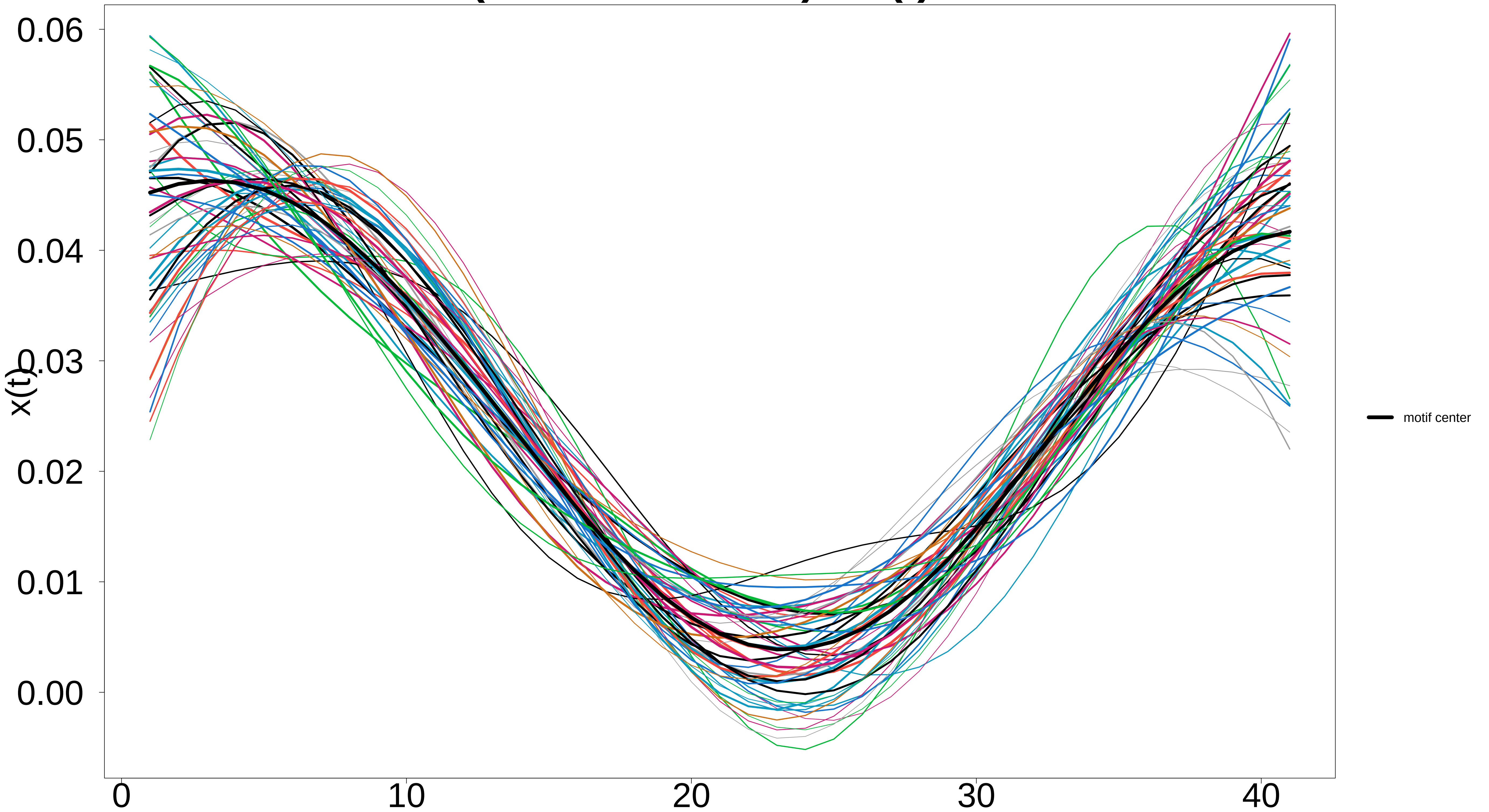
Motif 26 (52 occurrences) – x(t) derivative
