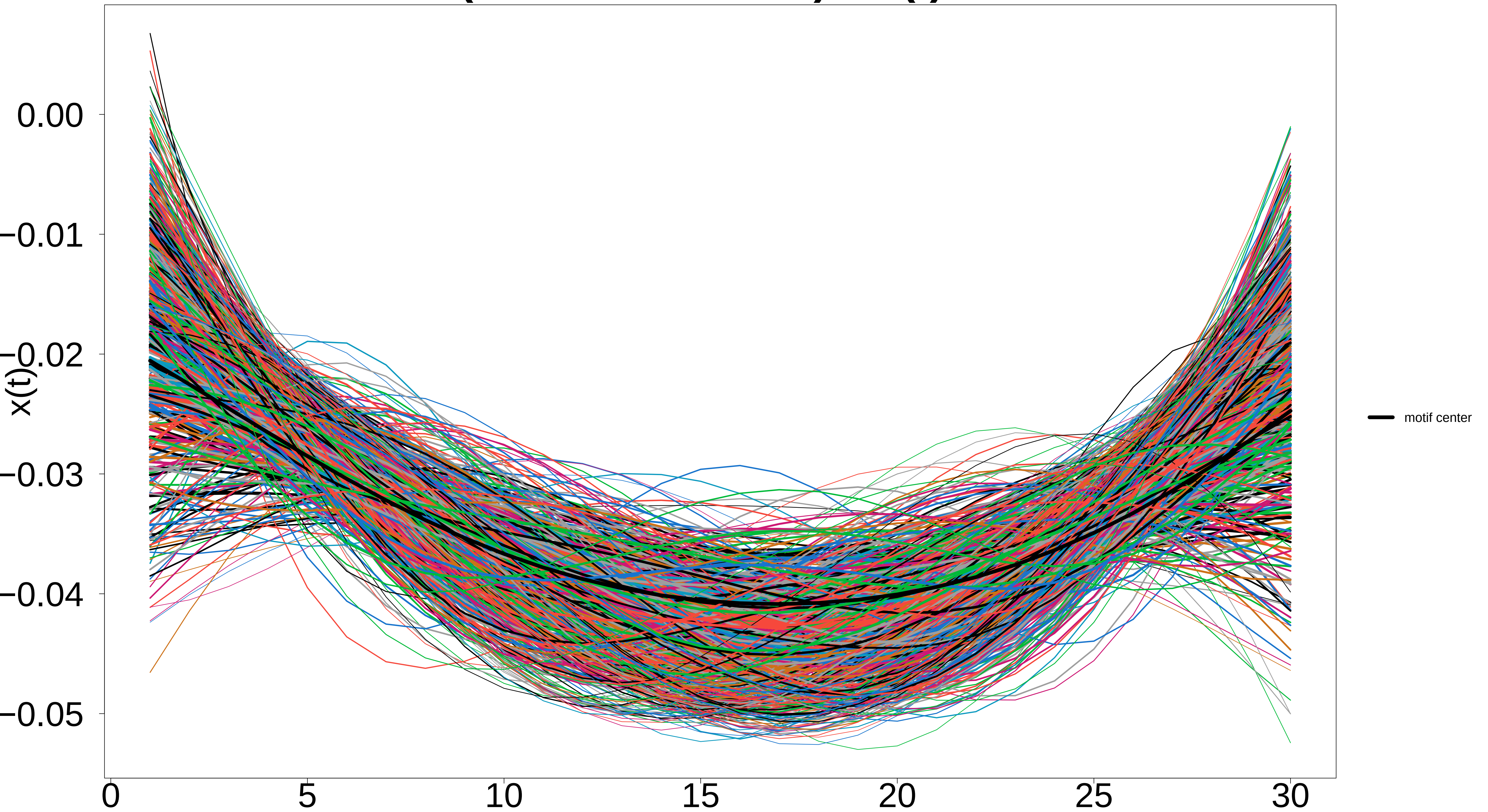
Motif 18 (580 occurrences) – x(t) derivative
