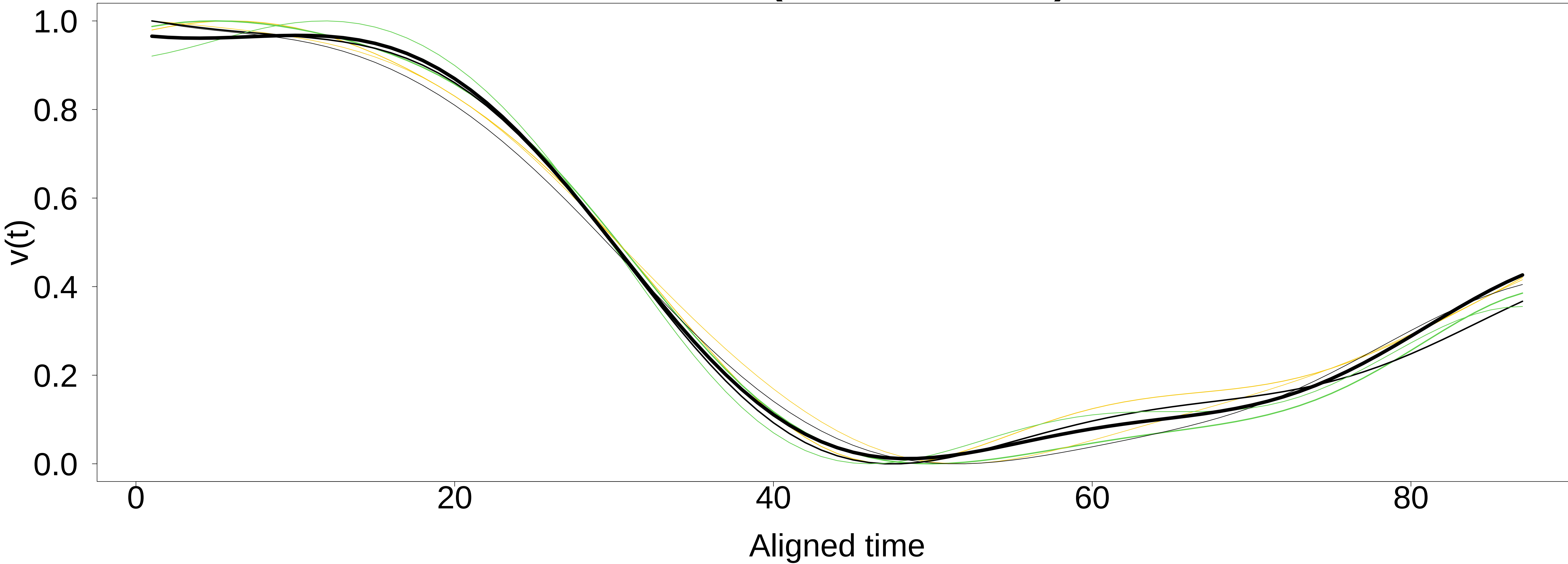
Motif 40 (6 occurrences)
