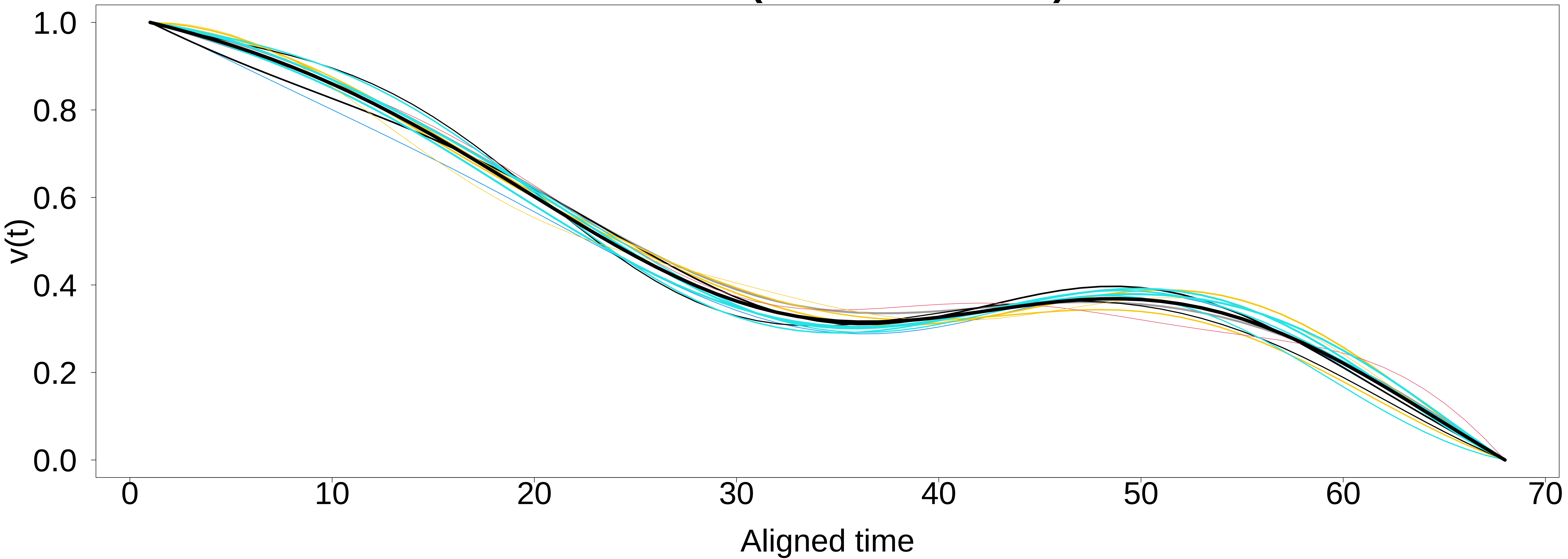
Motif 31 (12 occurrences)
