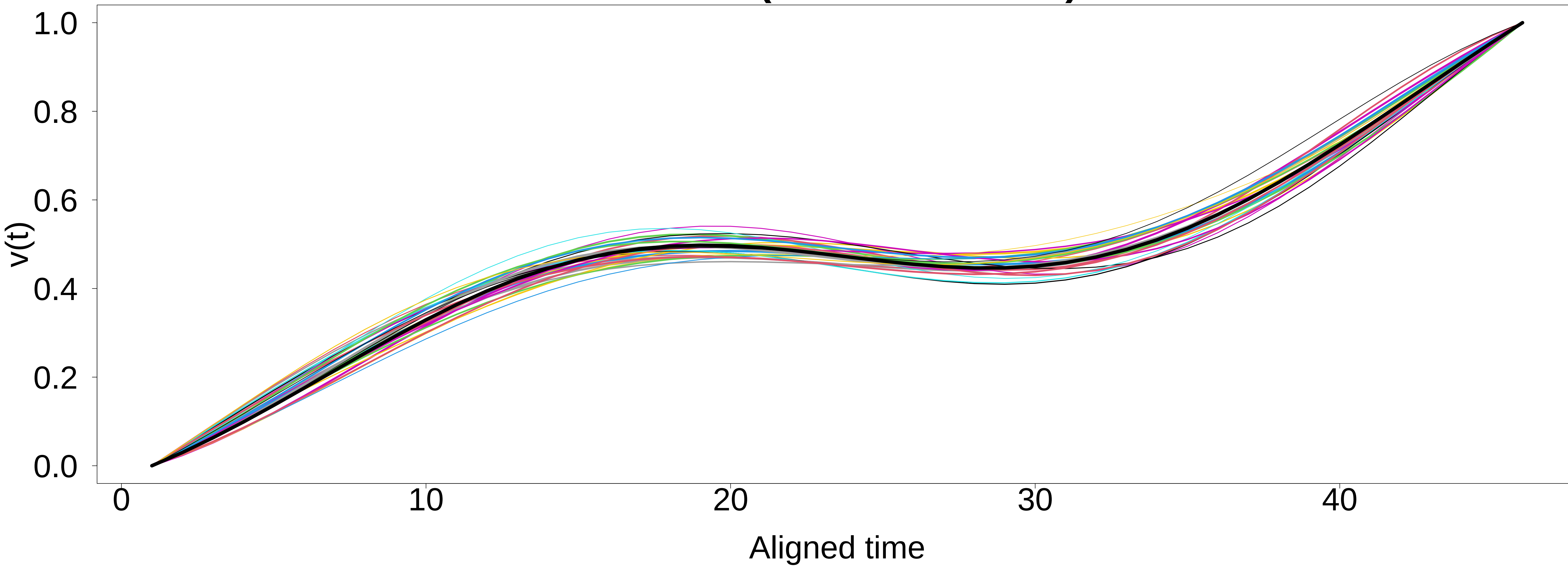
Motif 16 (27 occurrences)
