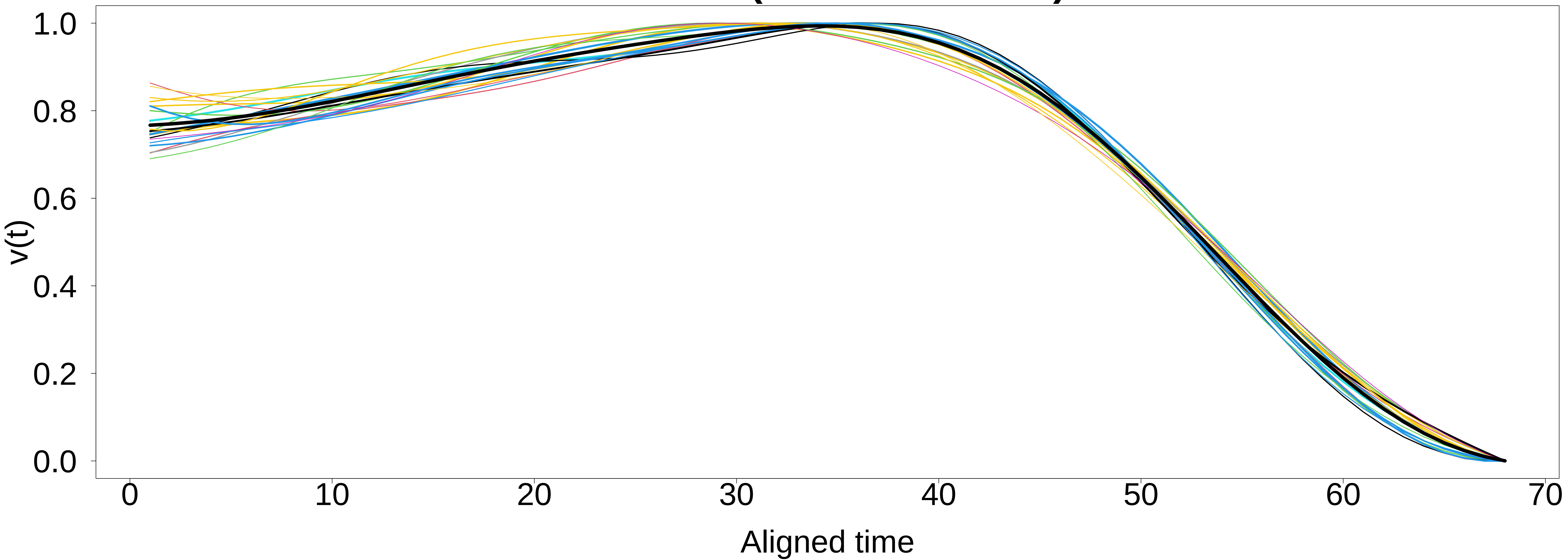
Motif 29 (20 occurrences)
