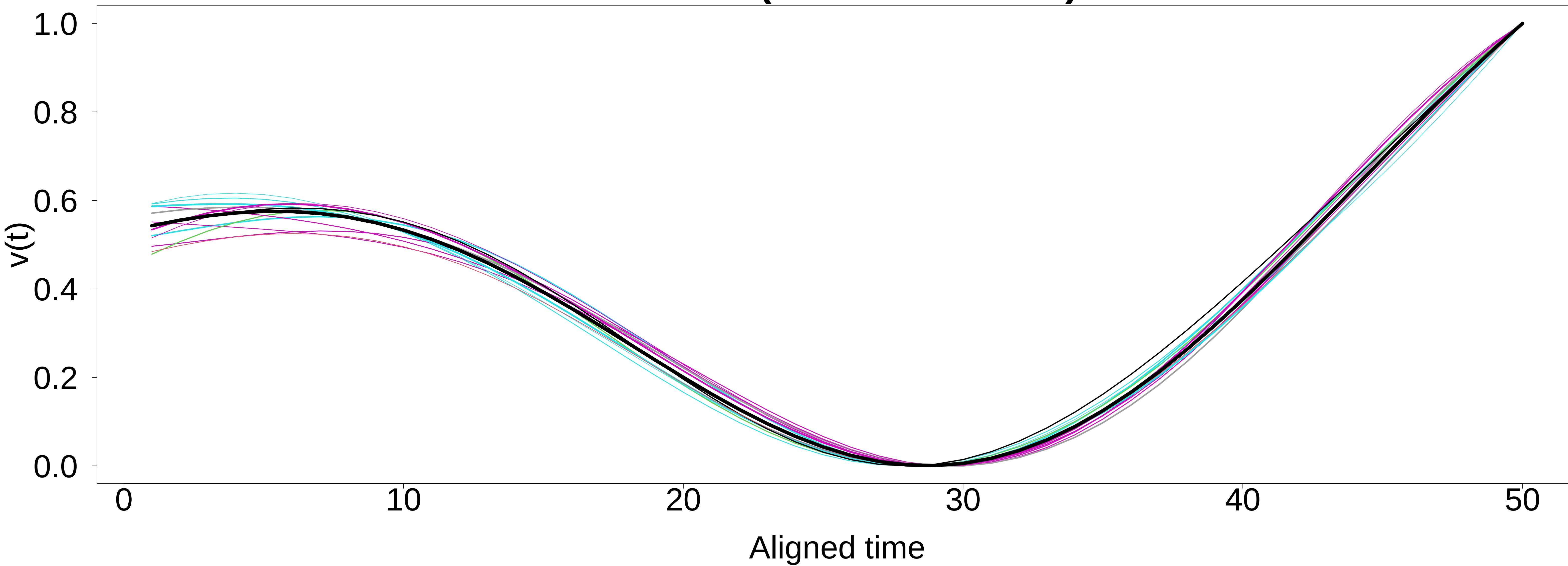
Motif 24 (13 occurrences)
