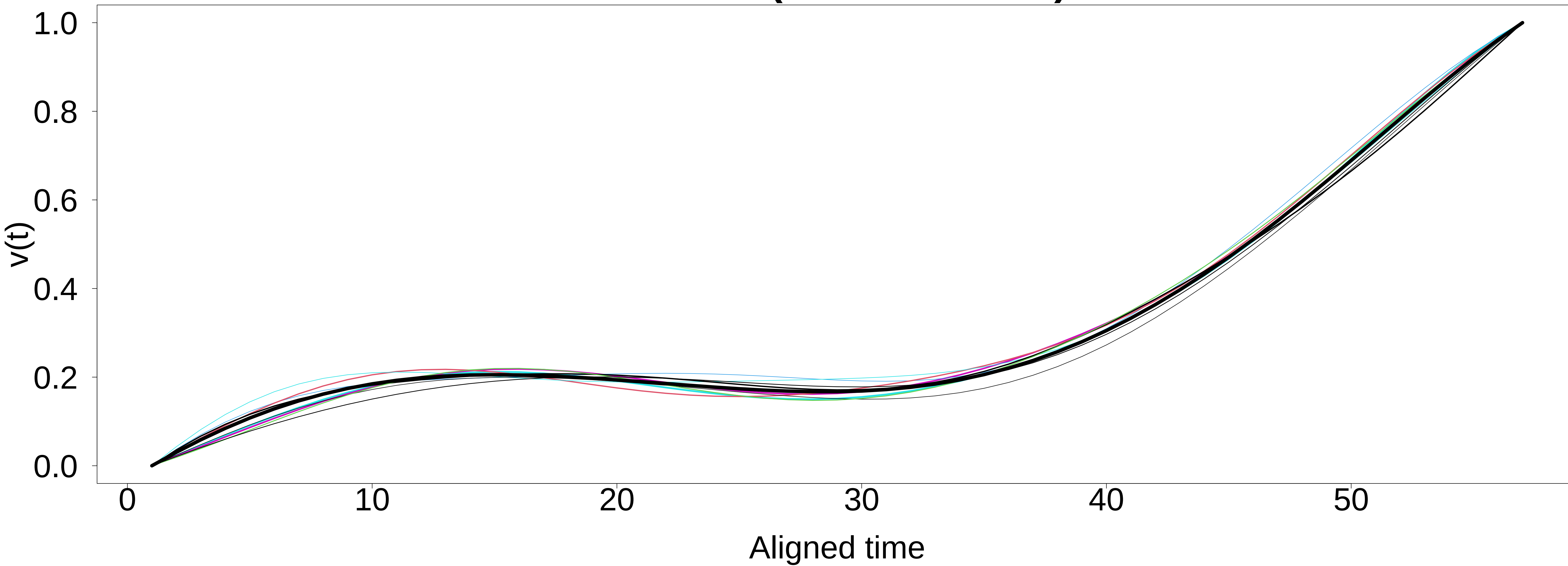
Motif 15 (9 occurrences)
