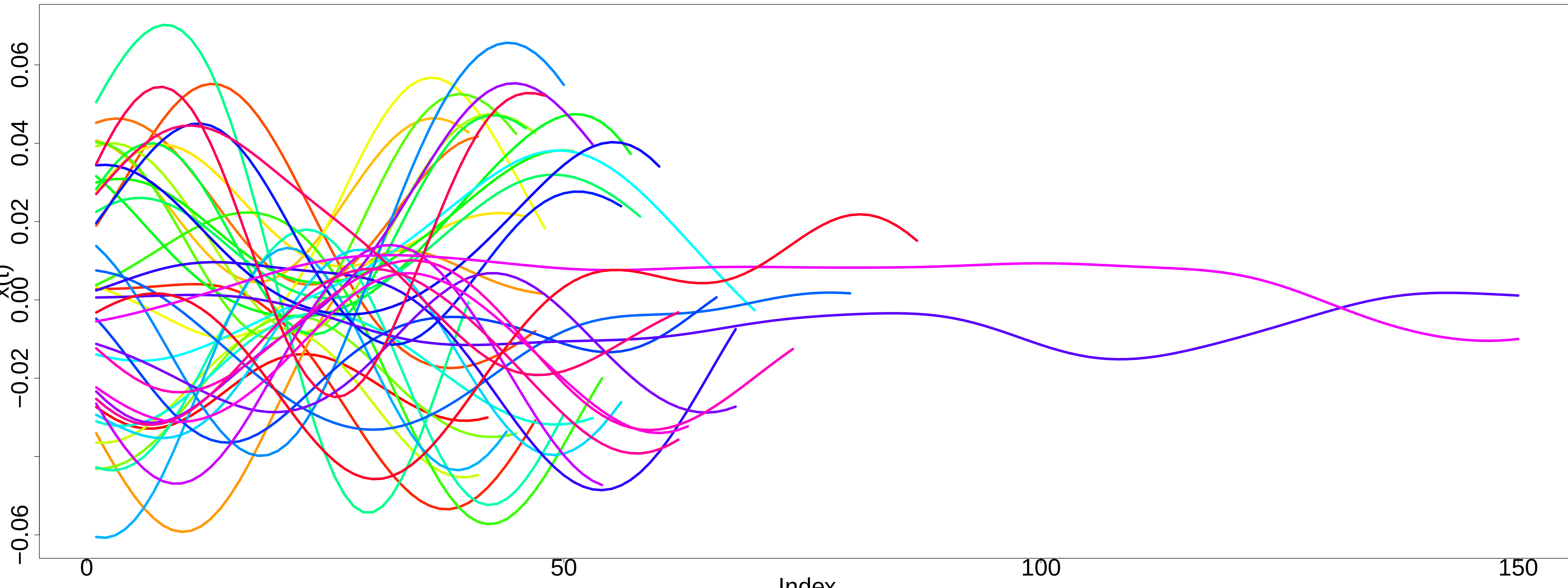
x(t) derivative
