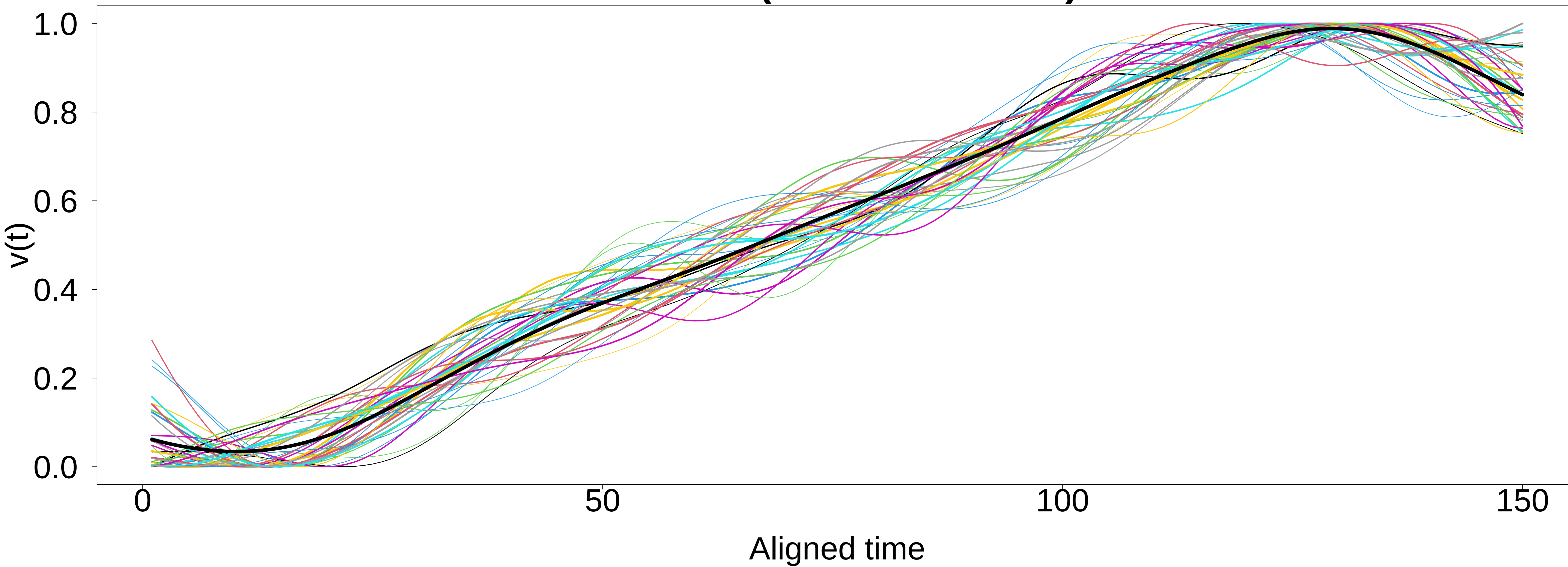
Motif 34 (37 occurrences)
