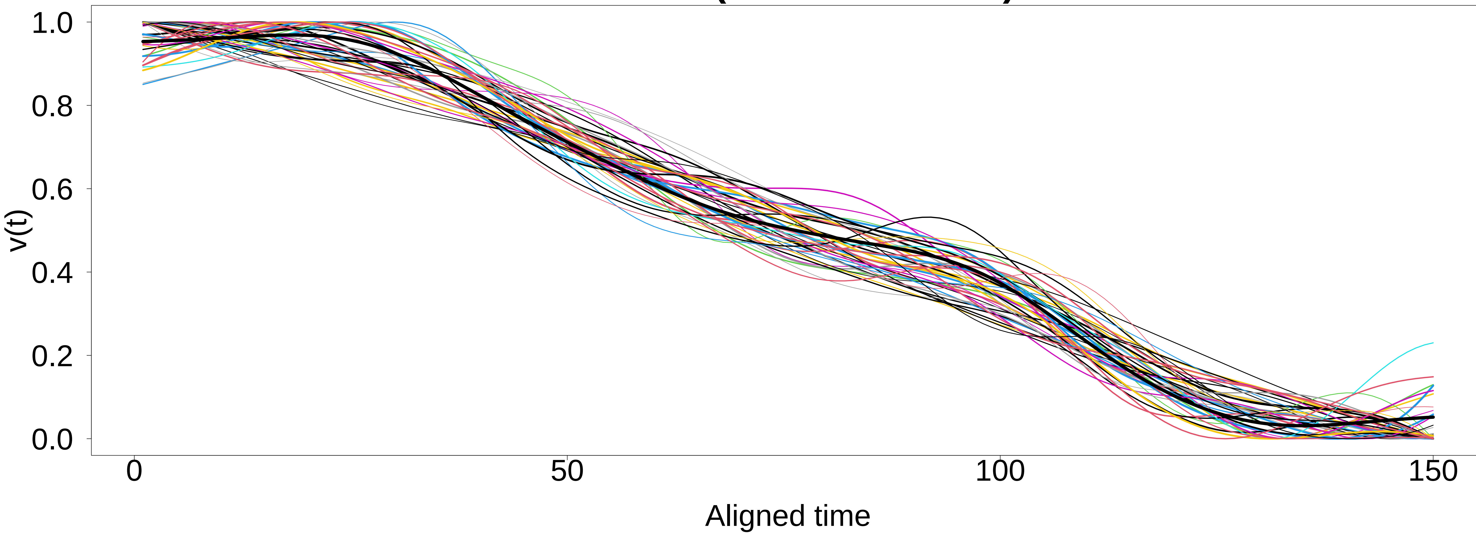
Motif 30 (43 occurrences)
