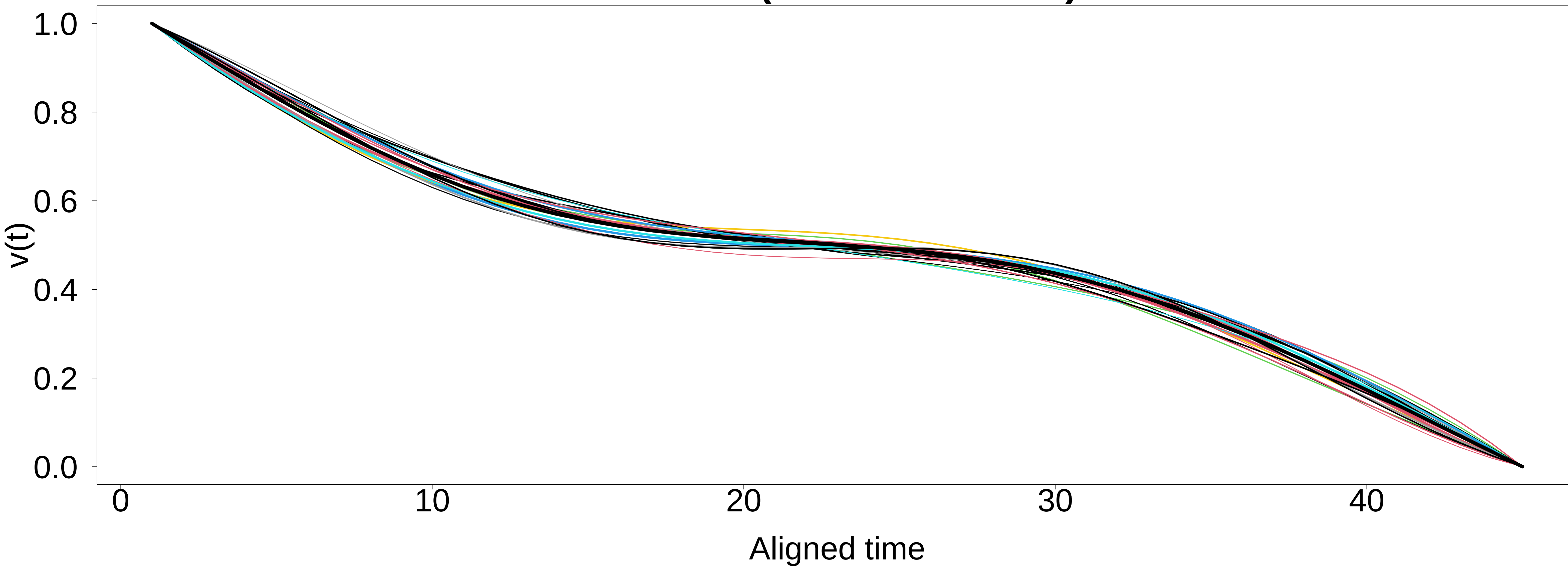
Motif 11 (22 occurrences)
