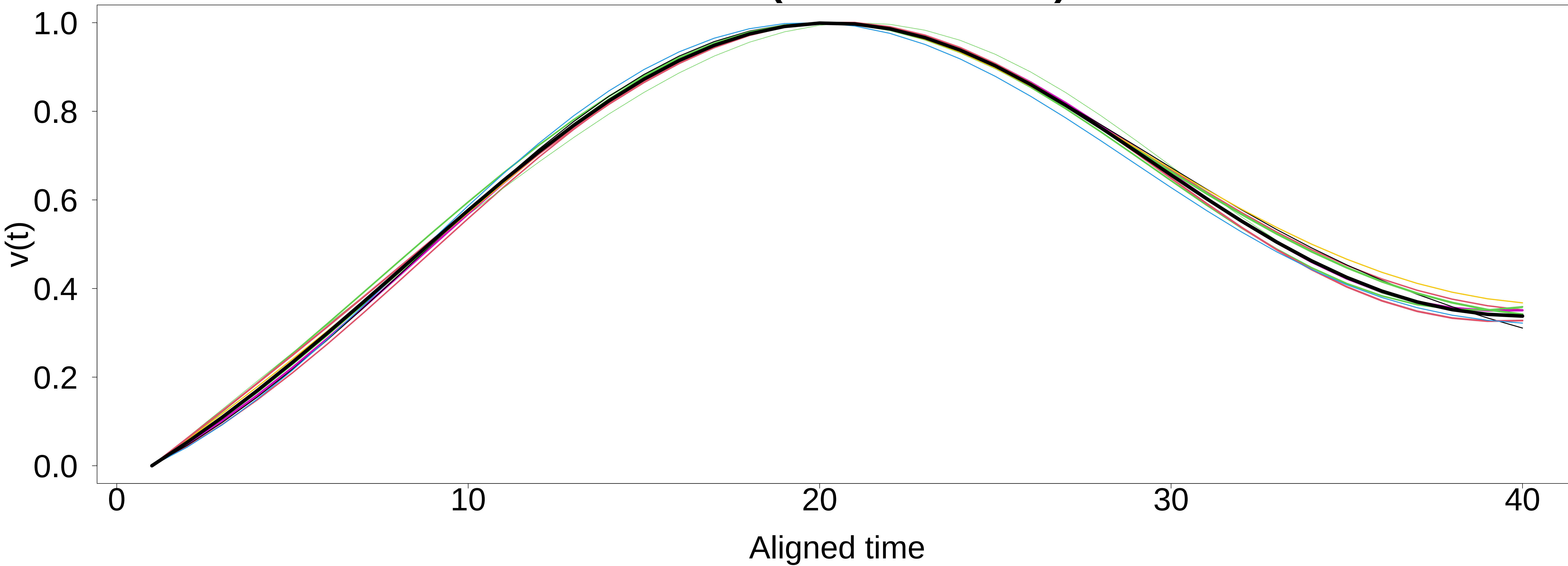
Motif 18 (9 occurrences)
