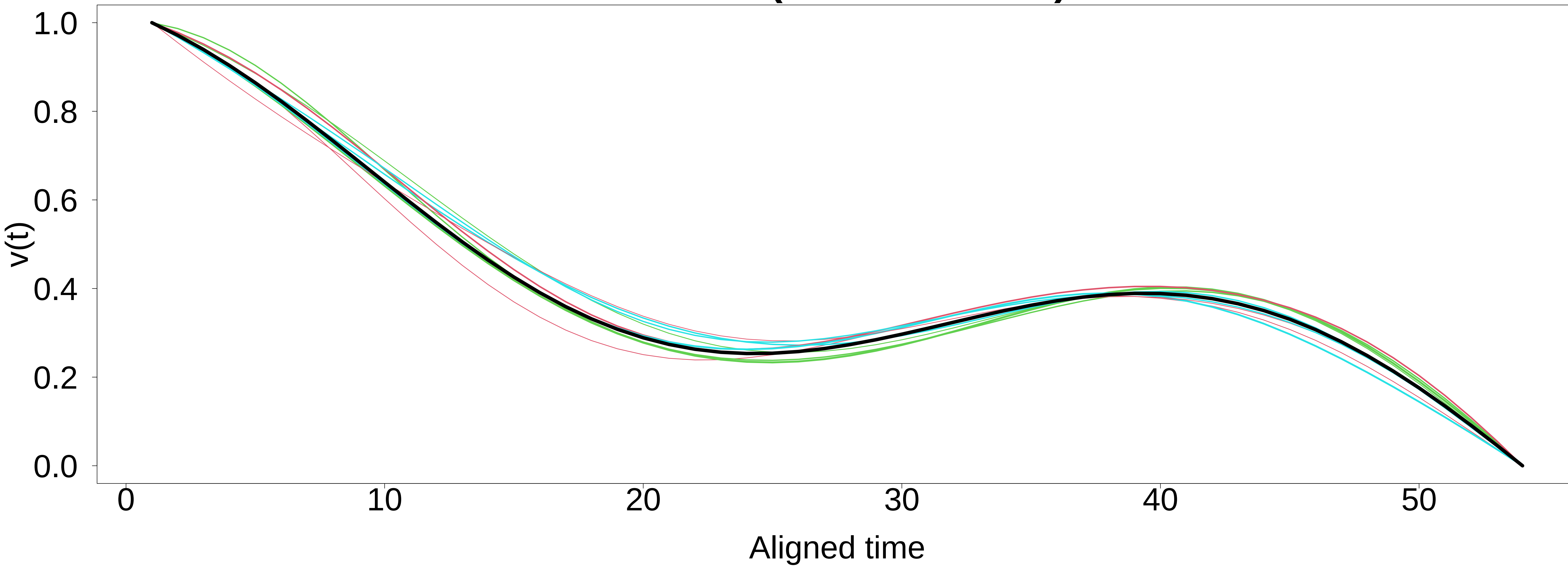
Motif 33 (9 occurrences)
