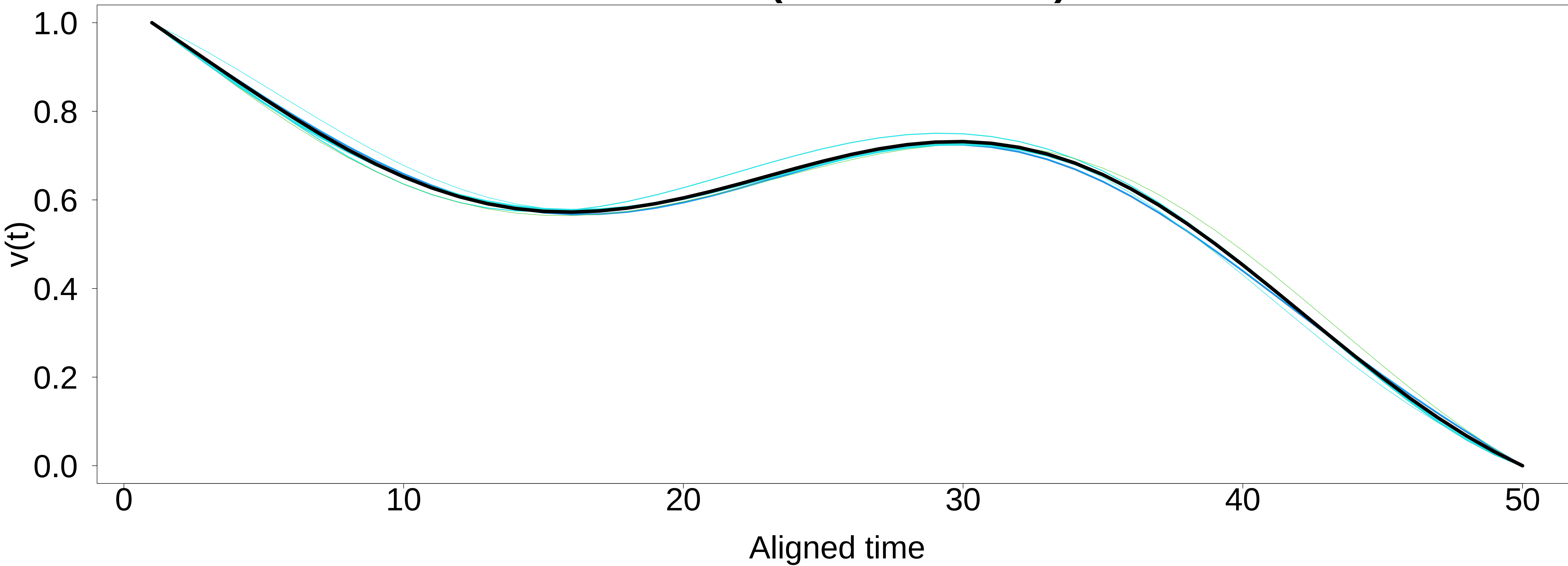
Motif 19 (5 occurrences)
