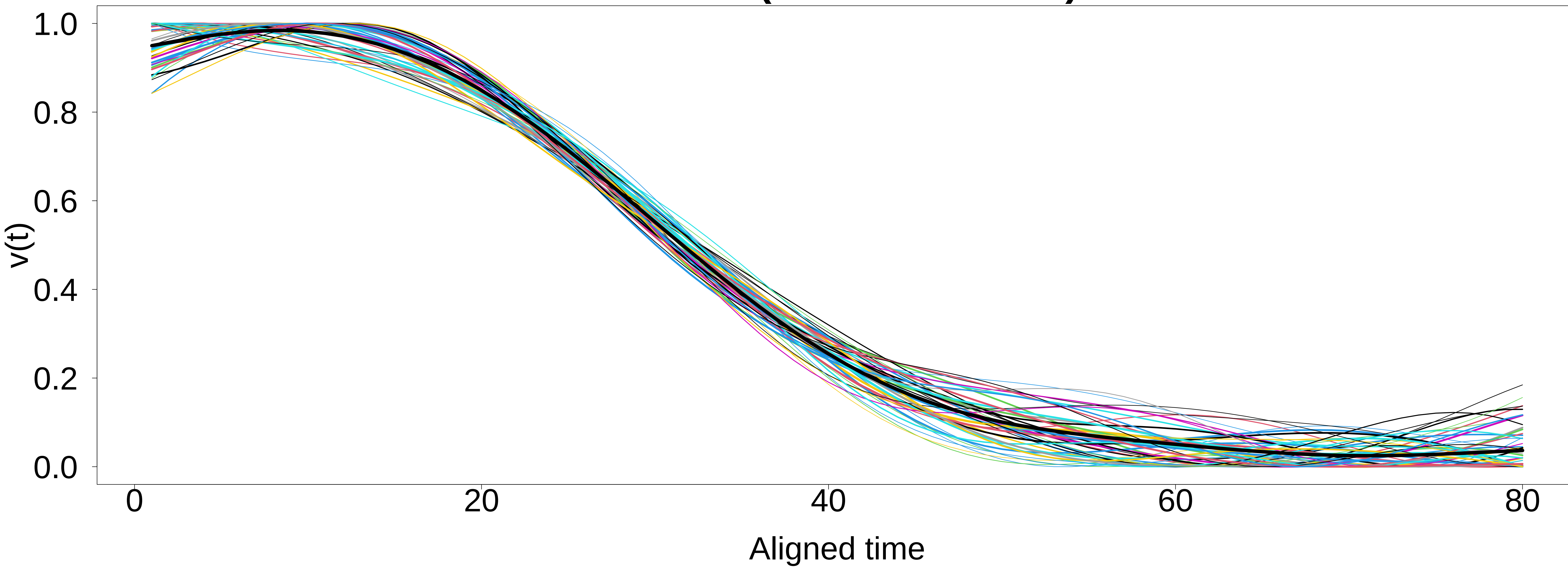
Motif 25 (47 occurrences)
