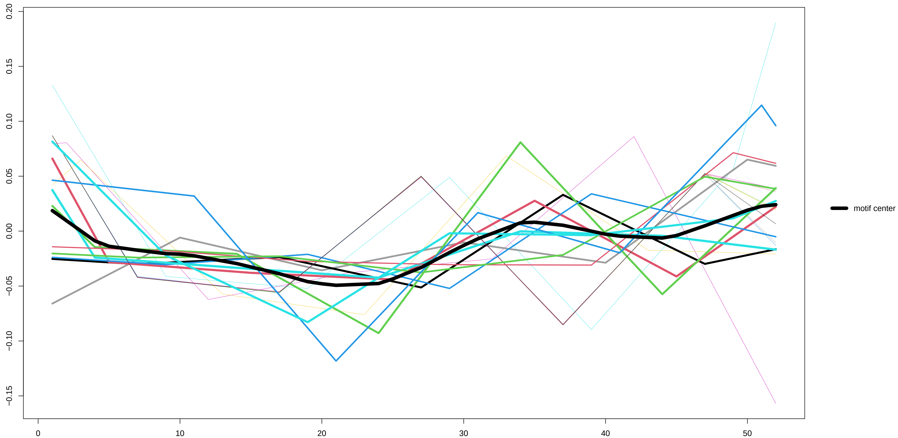
Motif 1 – derivative
