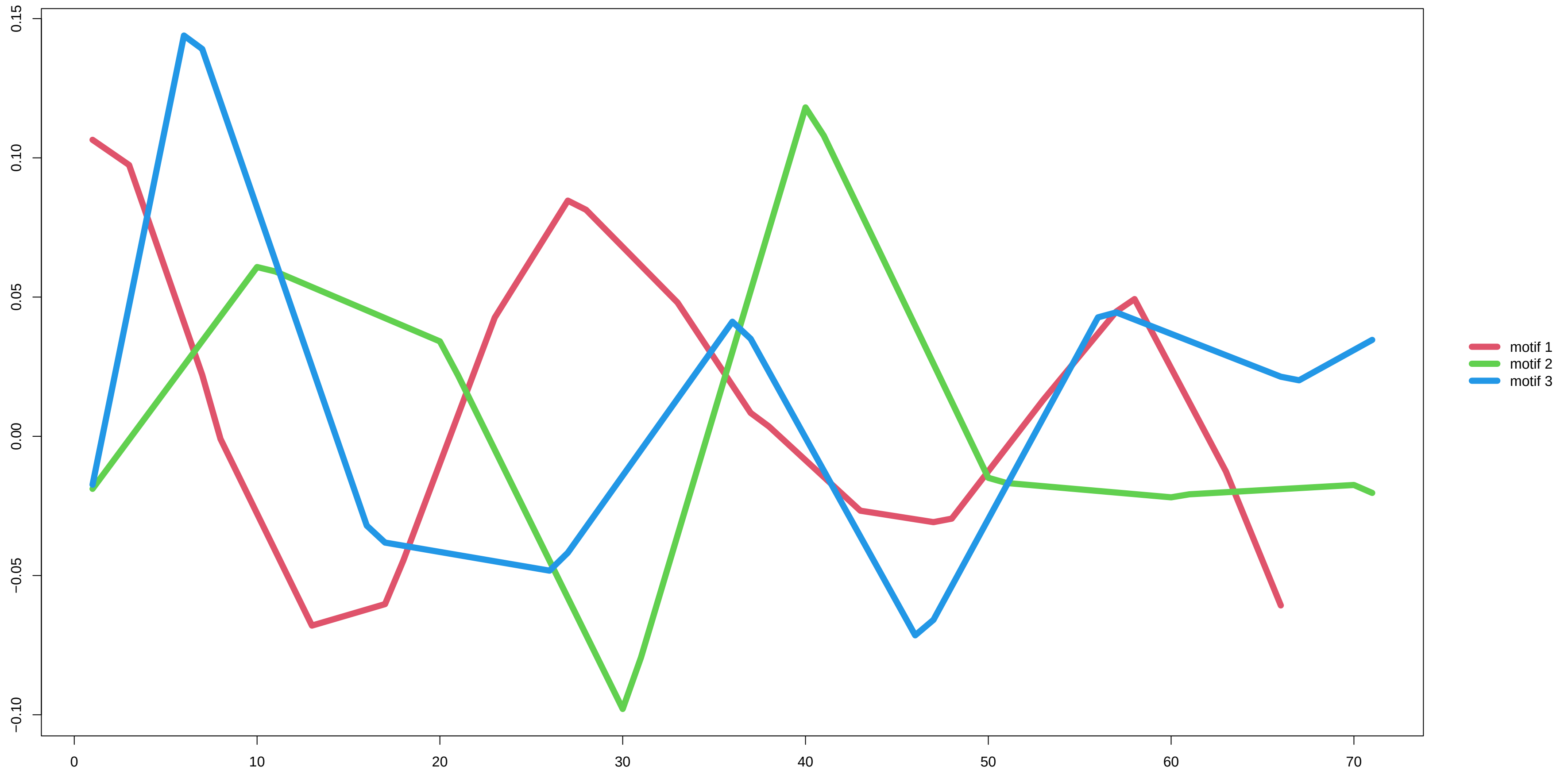
derivative
