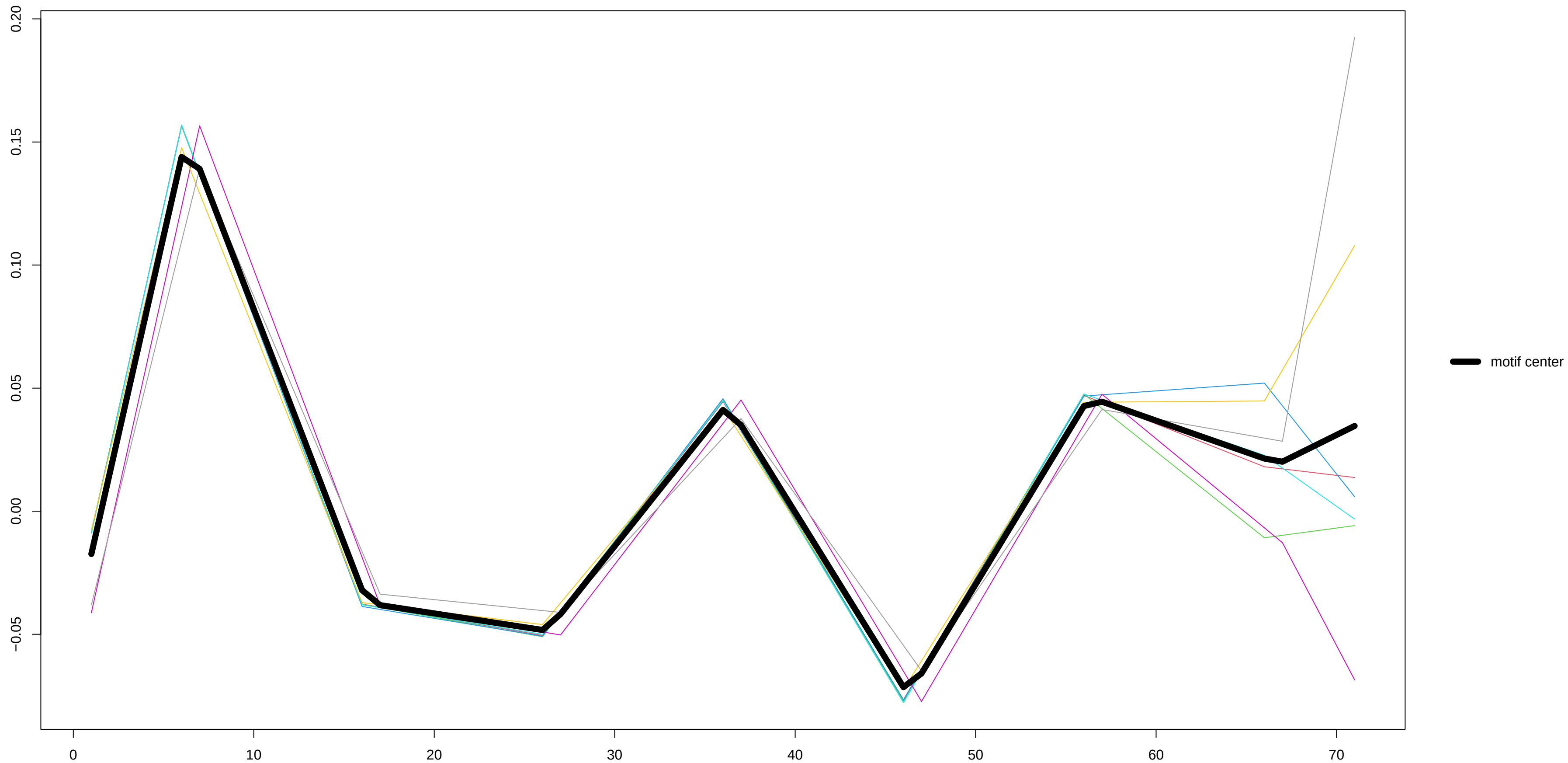
Motif 3 – derivative
