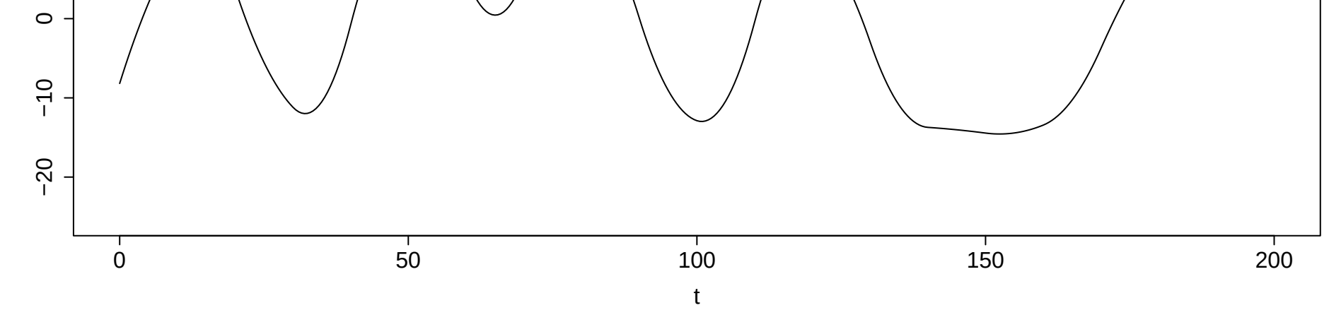
Random curve 15
