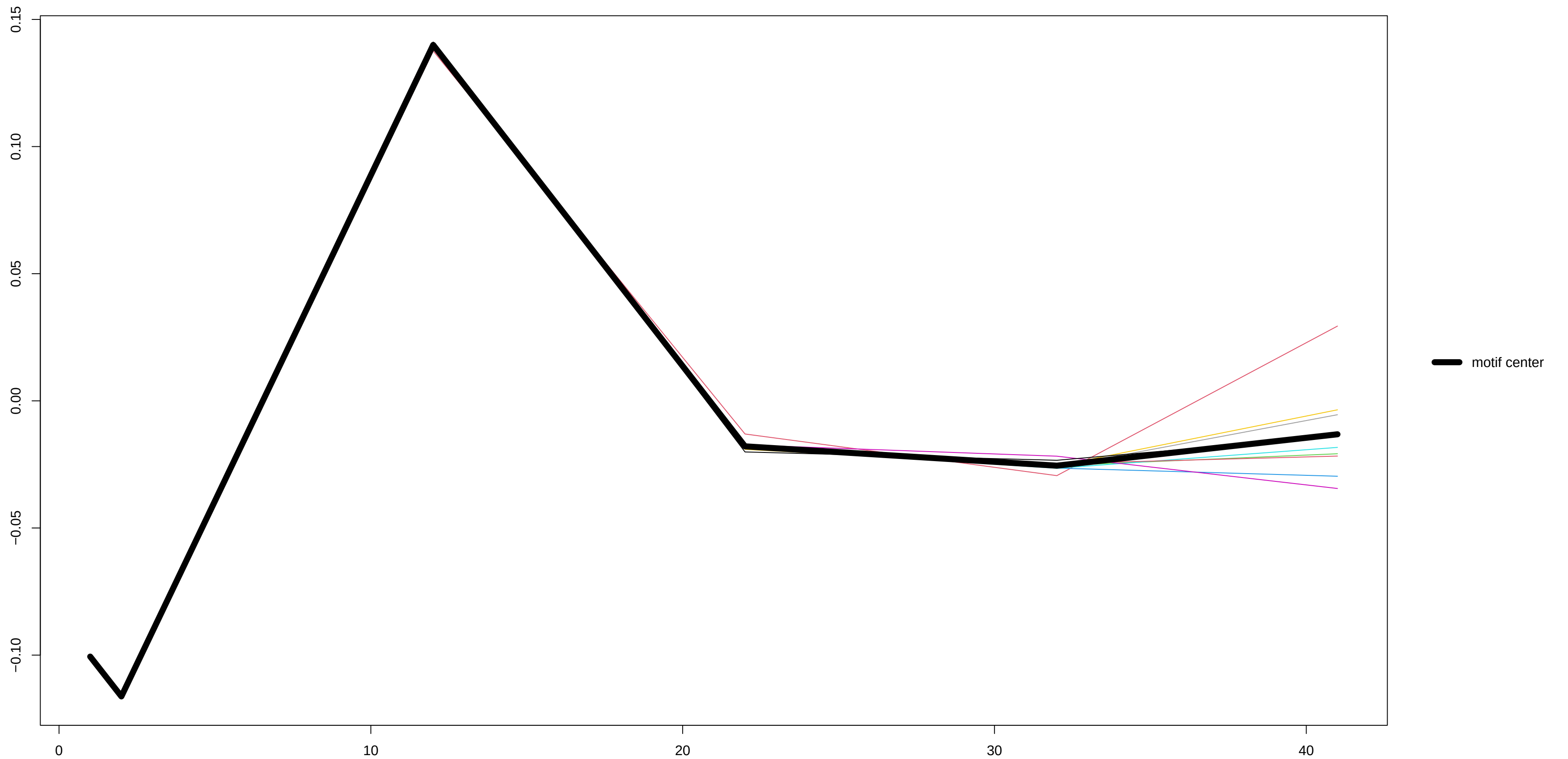
Motif 3 – derivative
