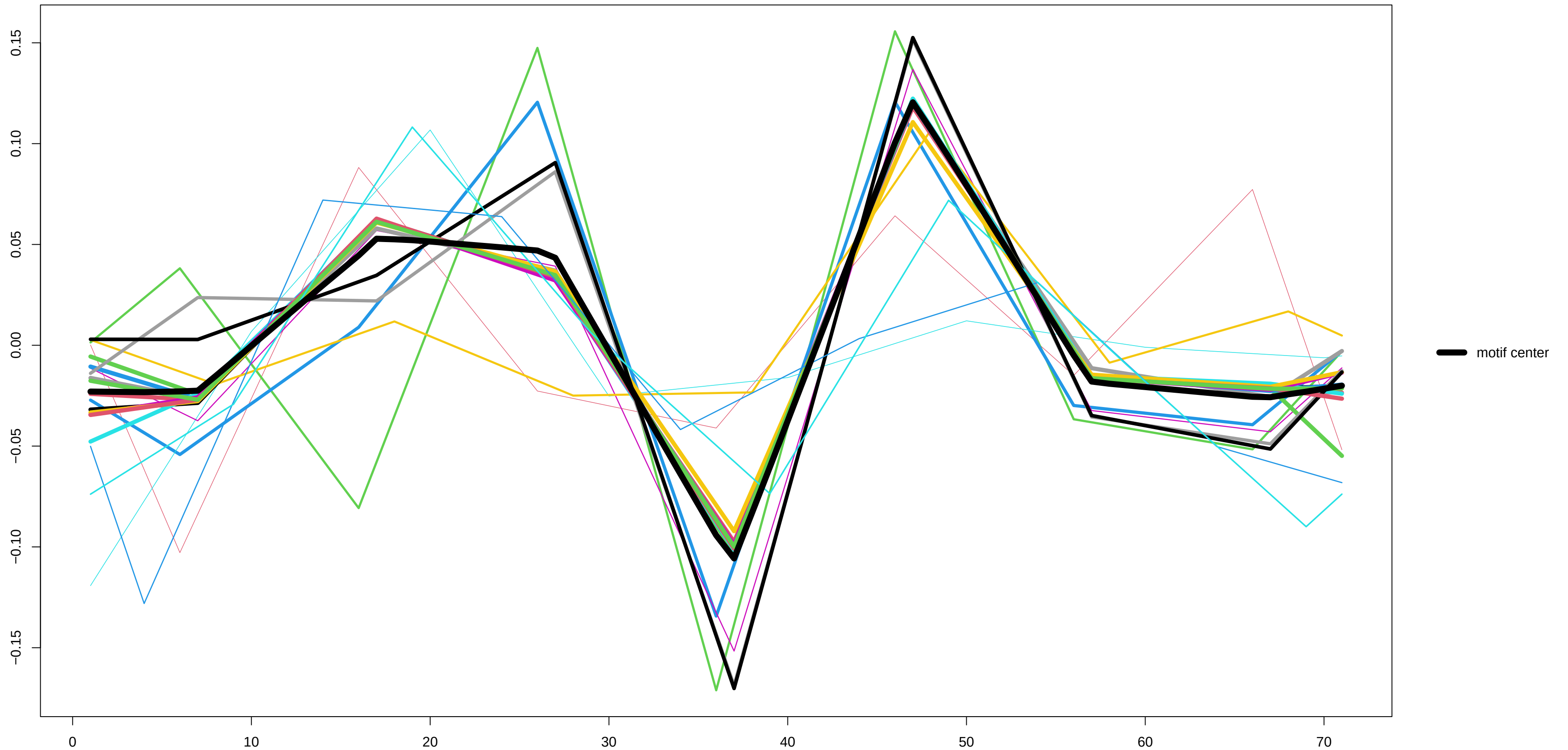
Motif 2 – derivative
