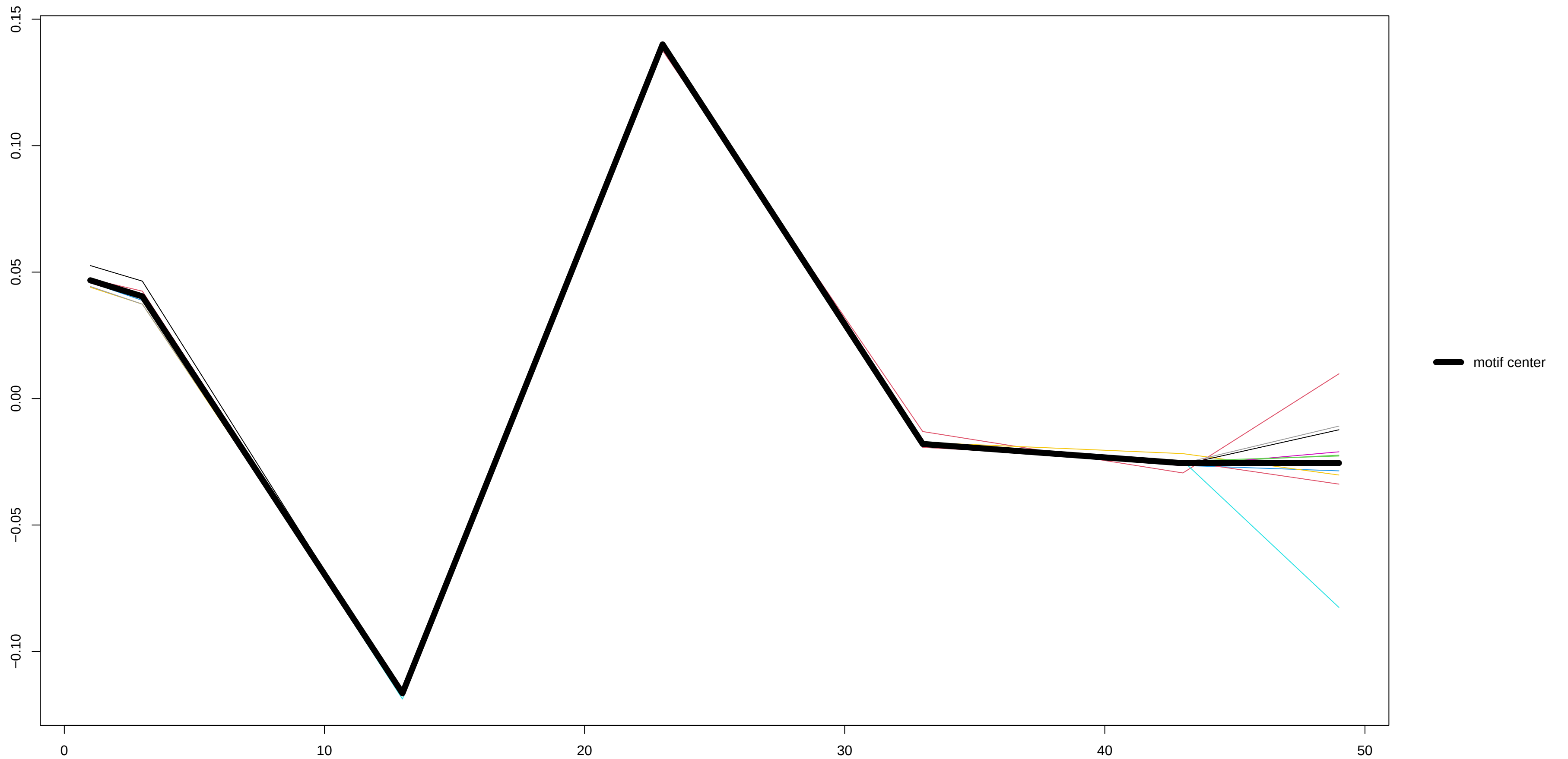
Motif 2 – derivative
