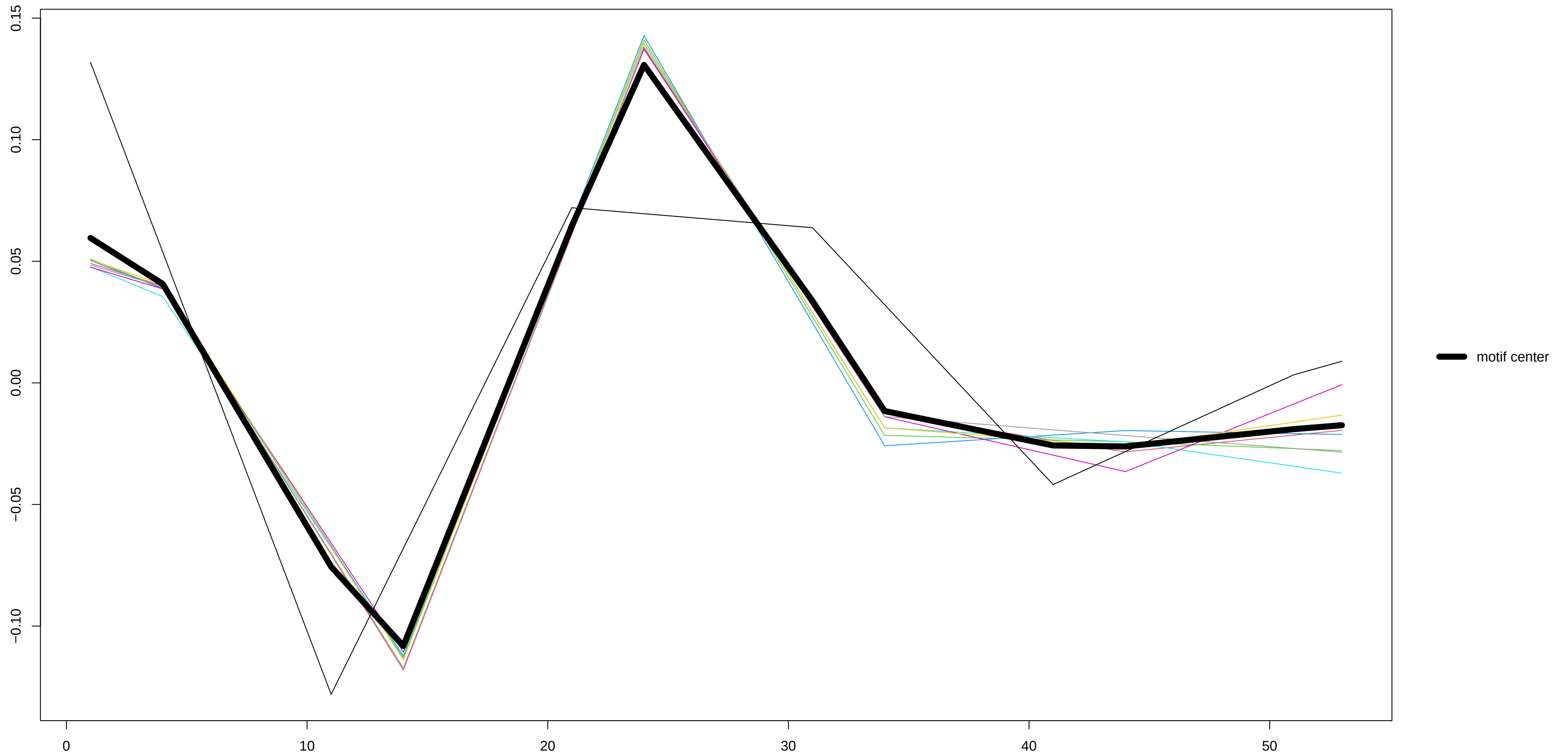
Motif 3 – derivative
