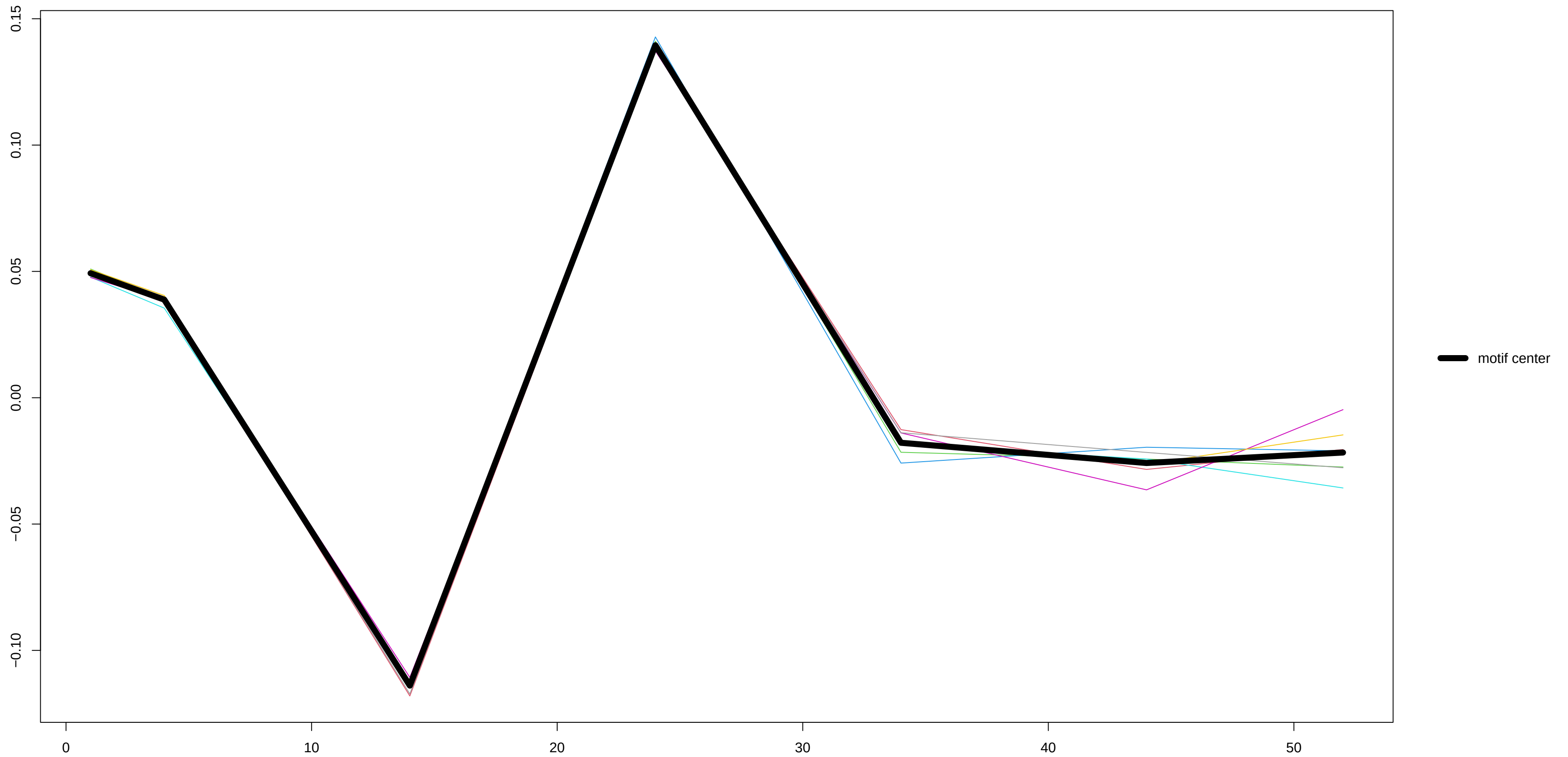
Motif 3 – derivative
