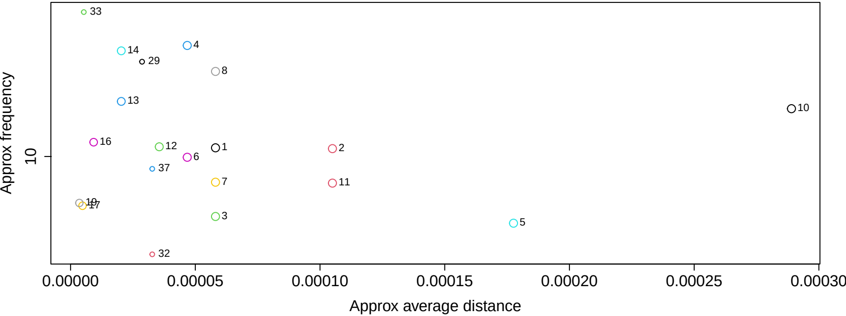
Motif in Cluster 1
