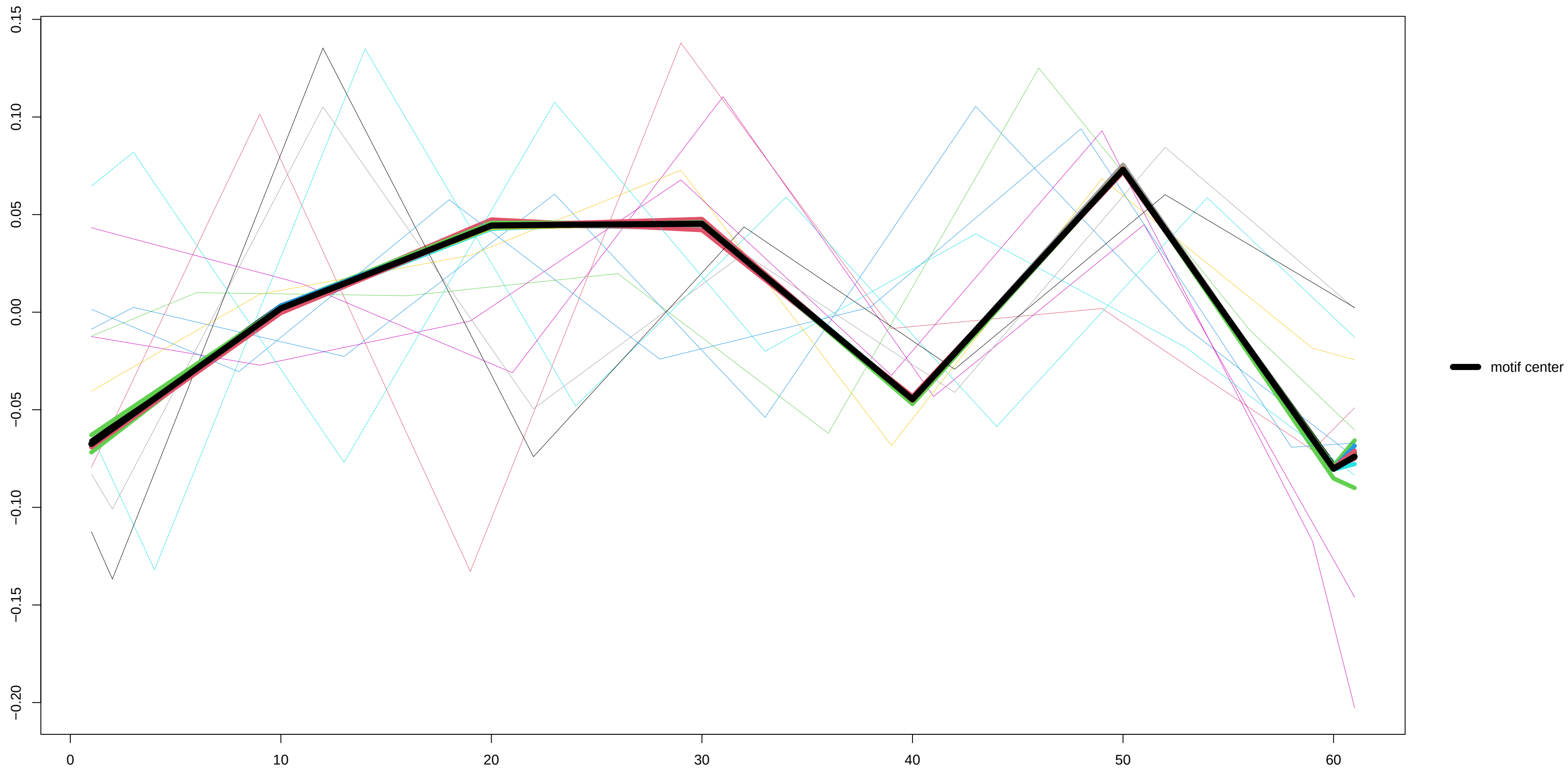
Motif 3 – derivative
