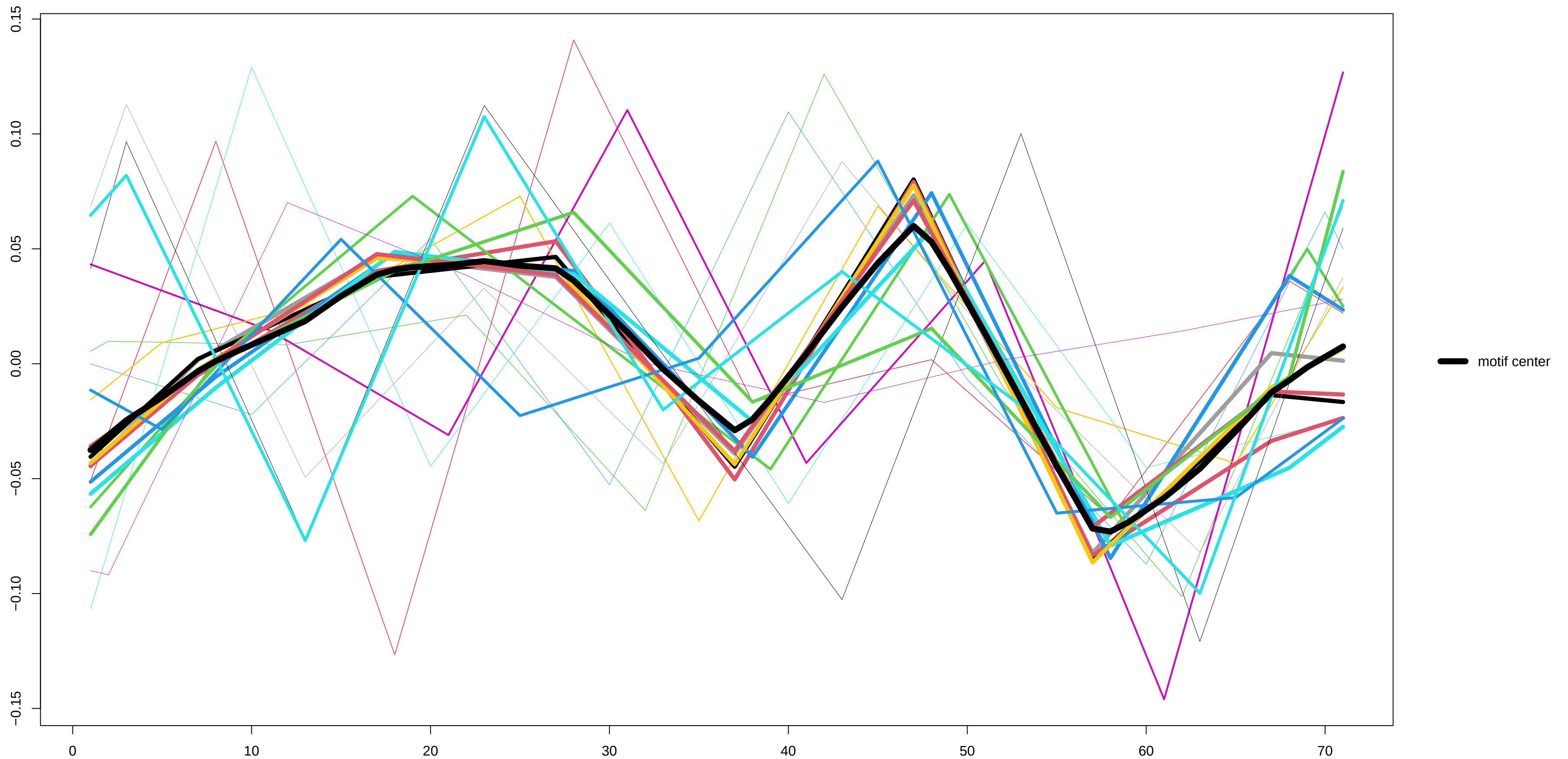
Motif 2 – derivative
