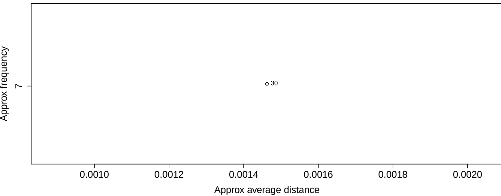
Motif in Cluster 4
