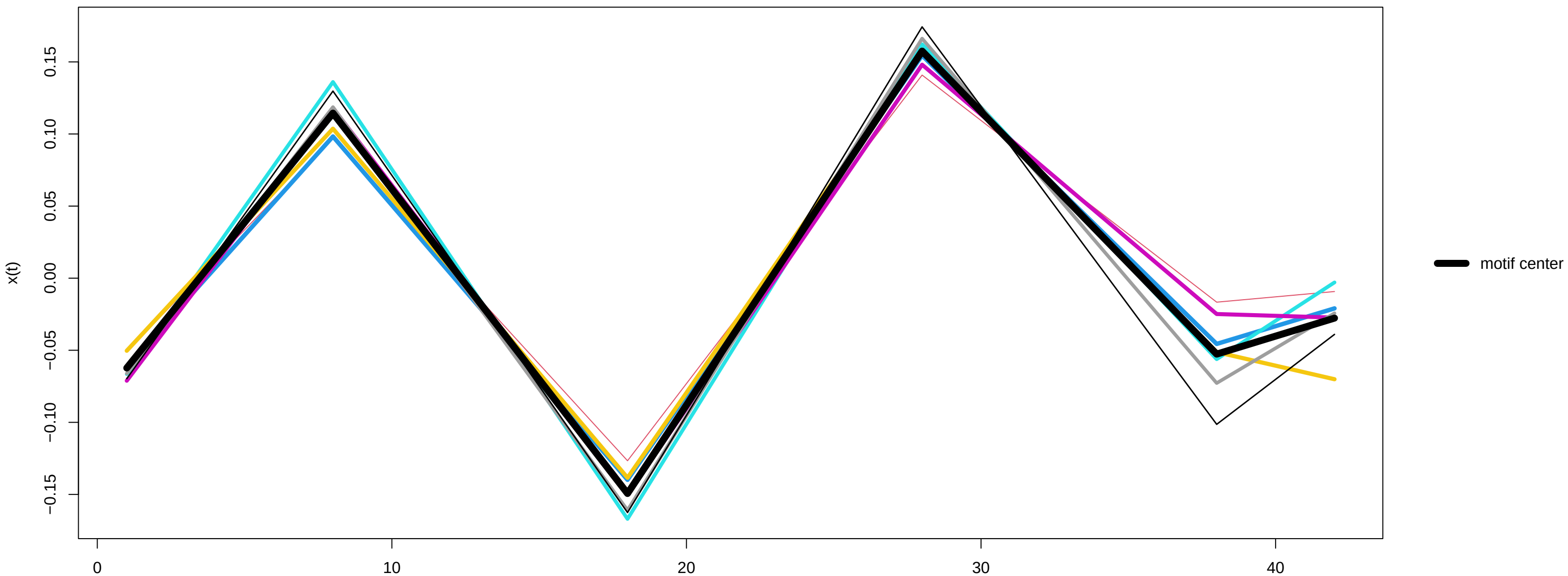
Motif 4 (7 occurrences) – x(t) derivative
