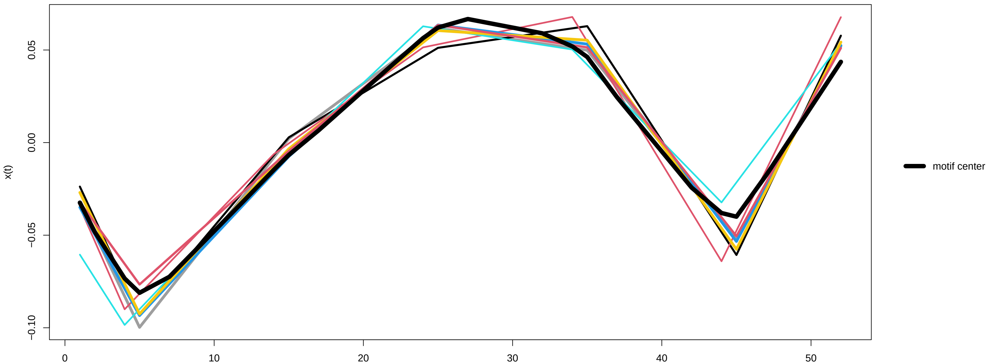
Motif 3 (7 occurrences) – x(t) derivative
