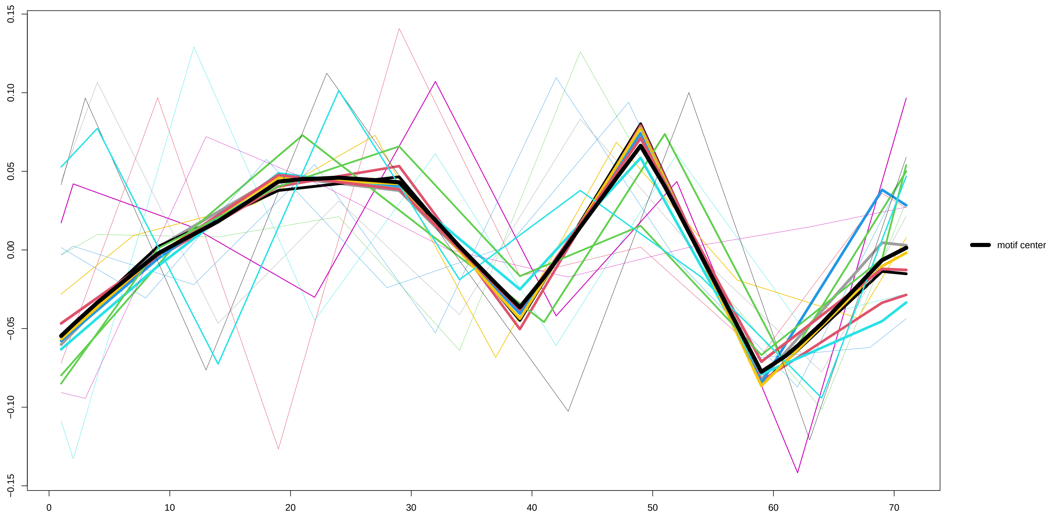
Motif 3 – derivative
