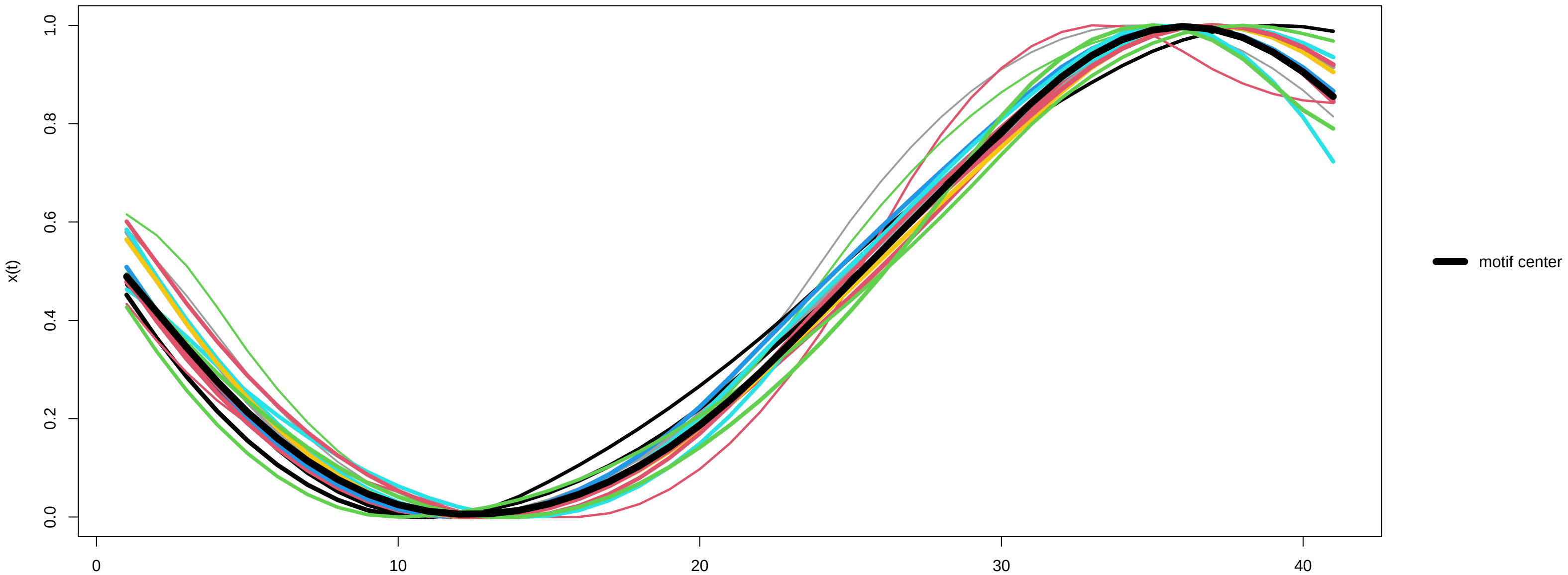
Motif 1 (15 occurrences) – x(t)
