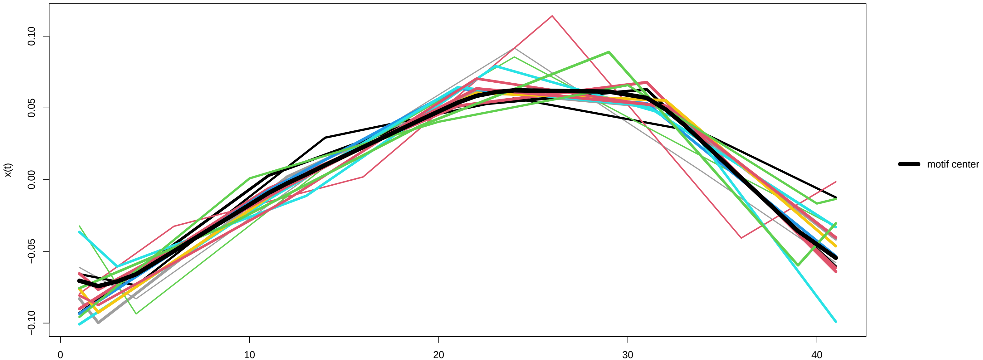
Motif 1 (15 occurrences) – x(t) derivative
