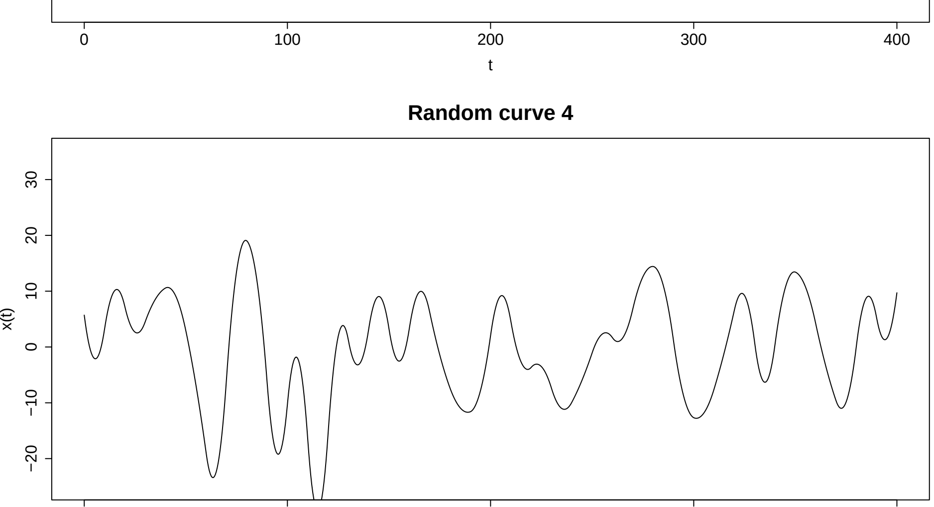
Random curve !
