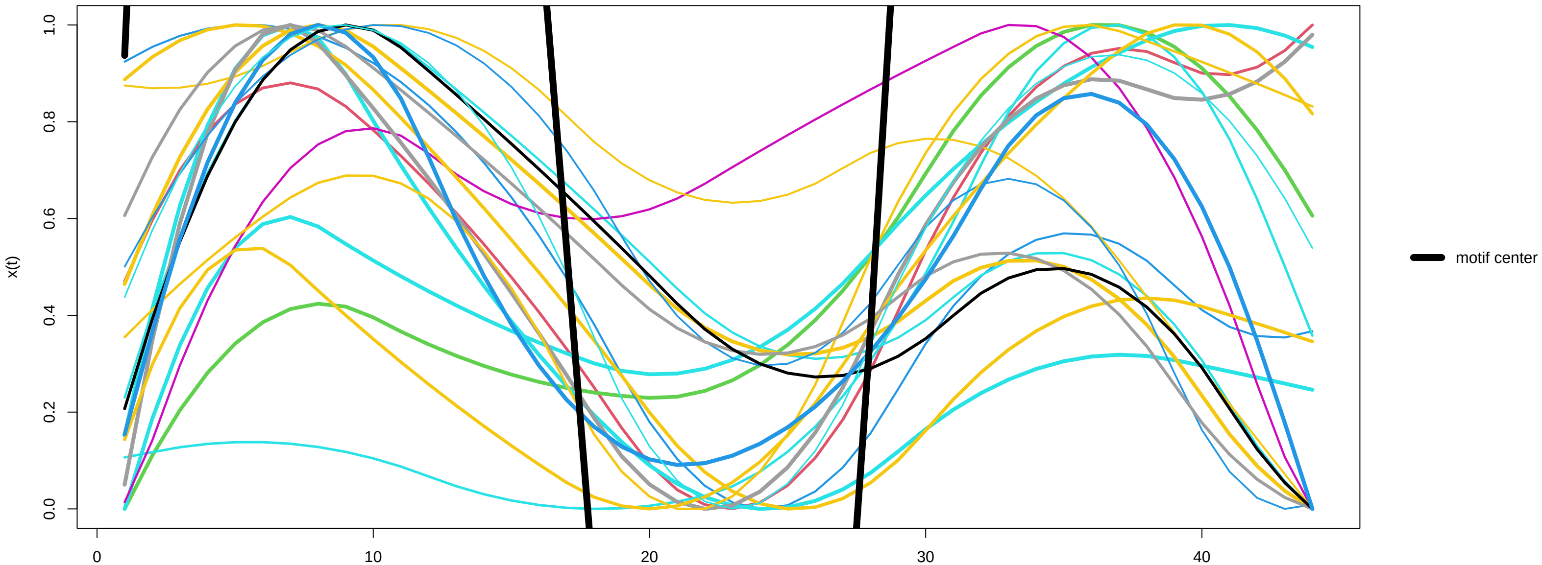
Motif 1 (19 occurrences) – x(t)
