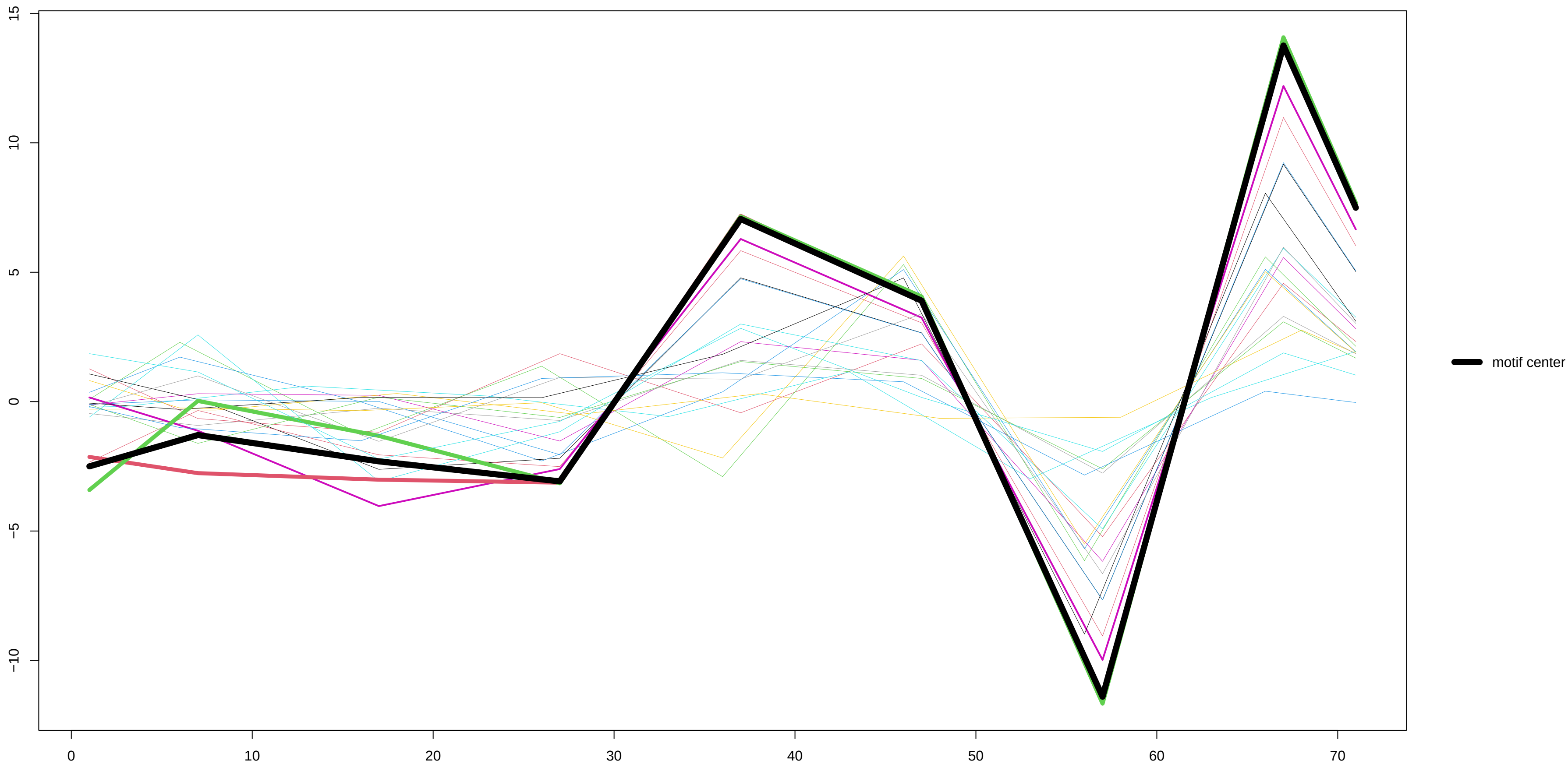
Motif 1 – derivative
