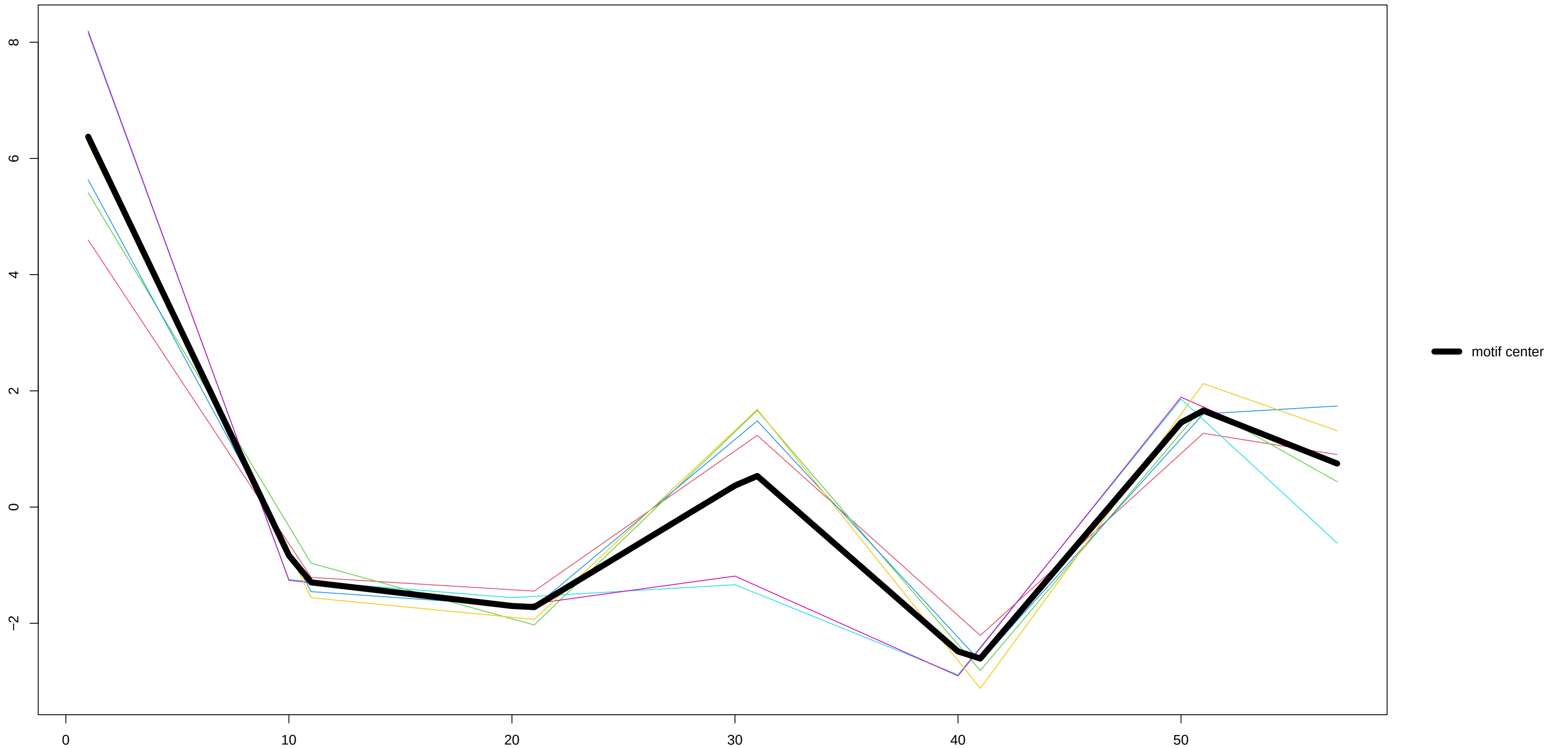
Motif 1 – derivative
