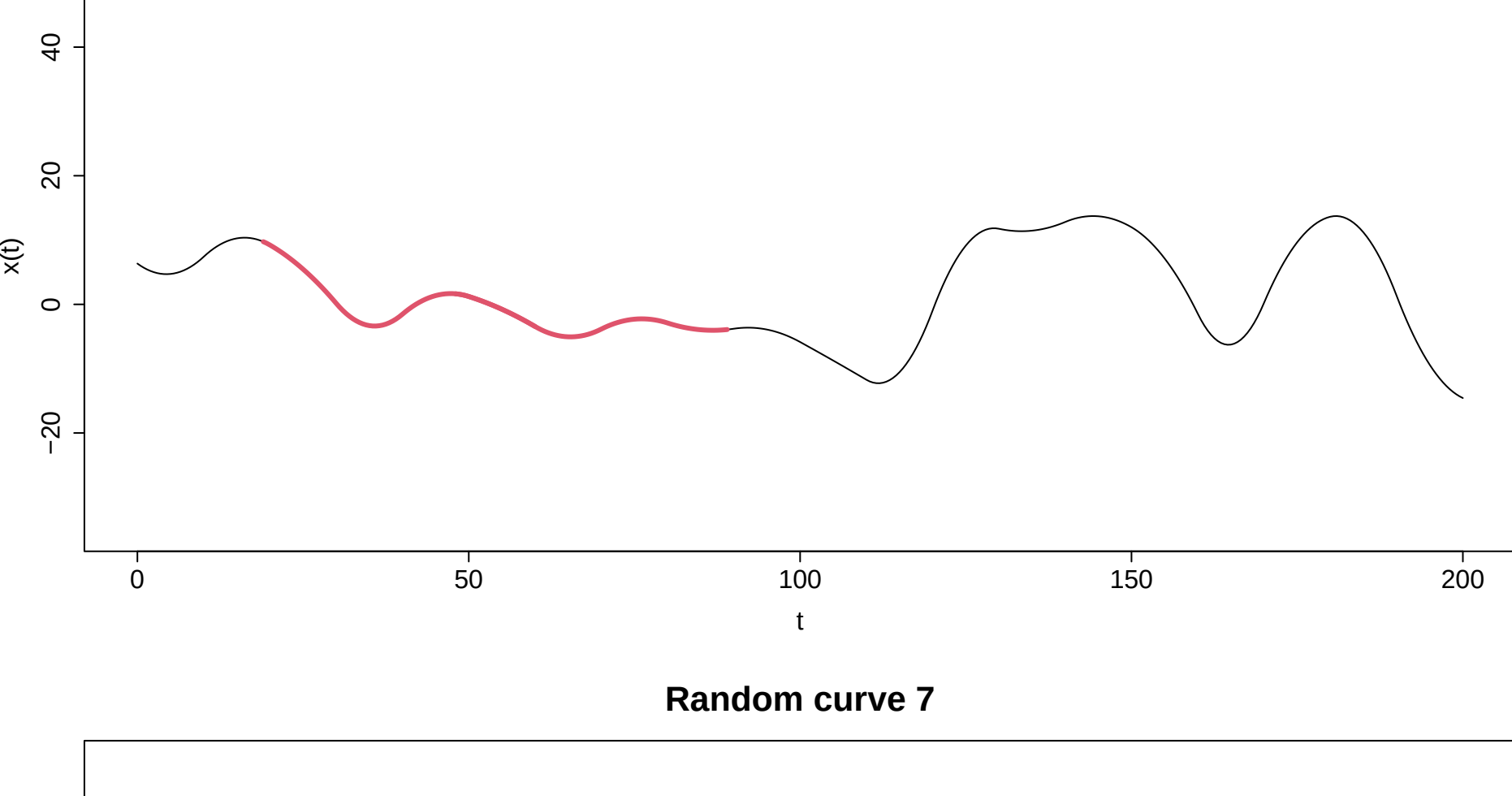
Random curve 6
