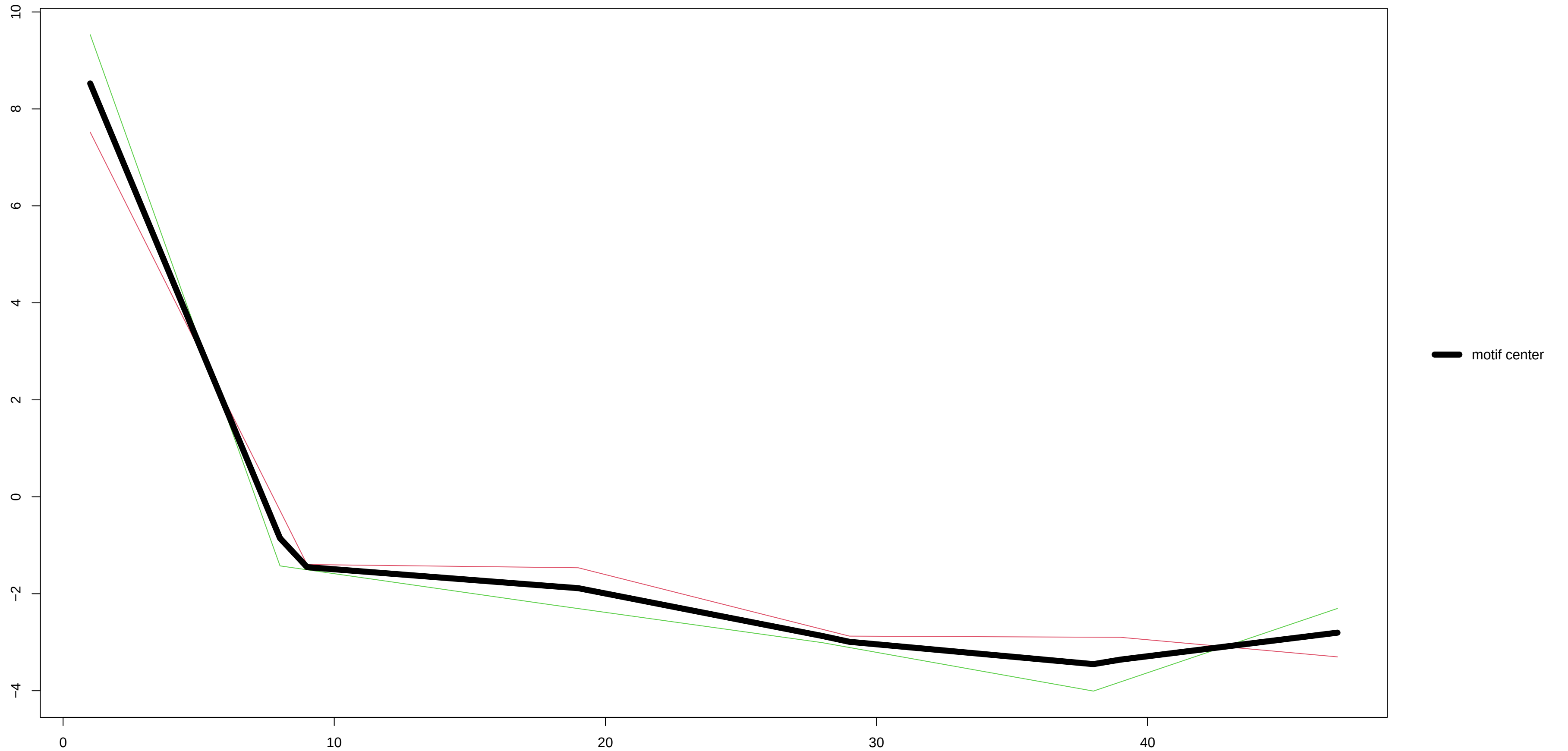
Motif 3 – derivative
