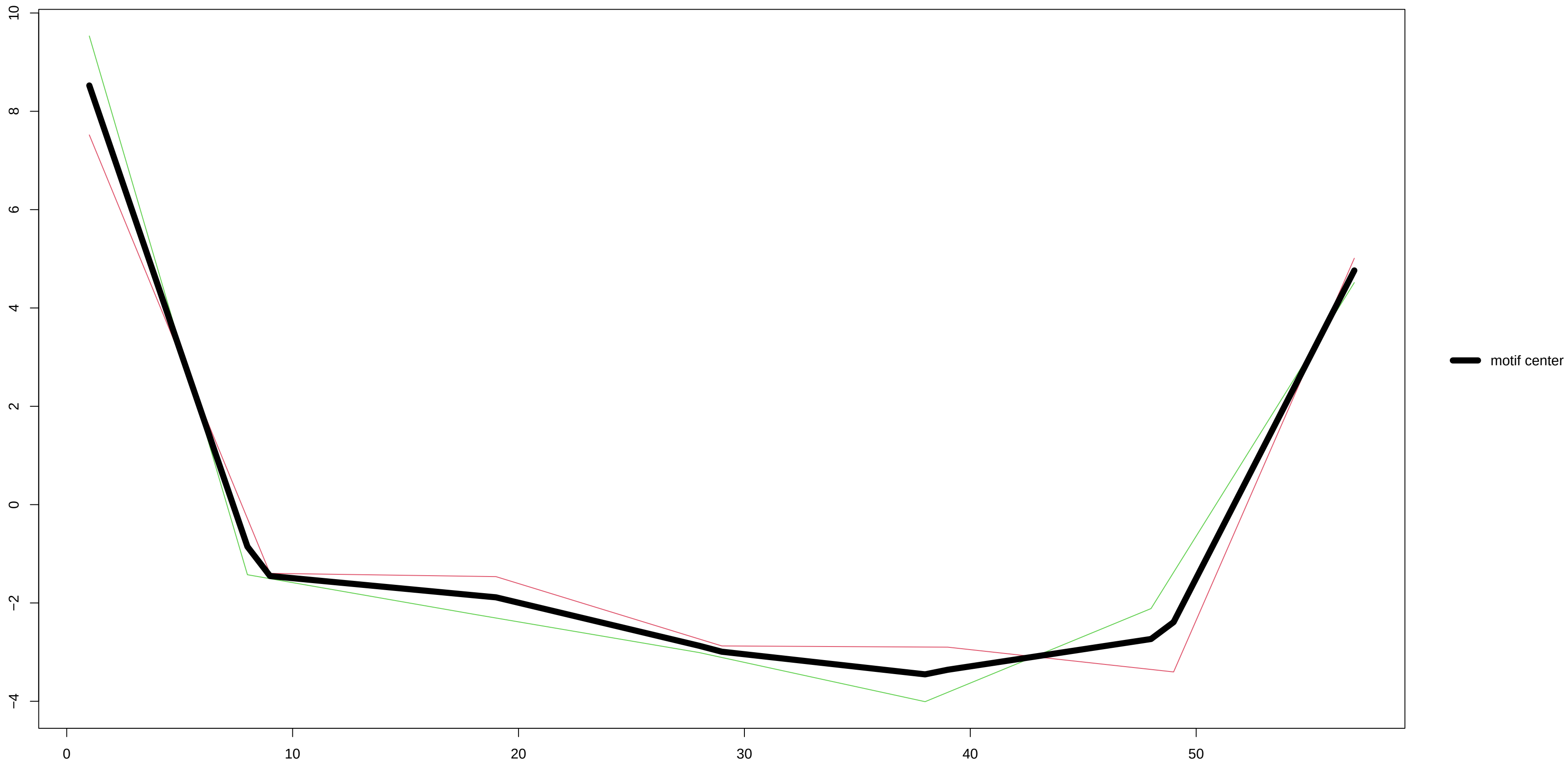
Motif 1 – derivative
