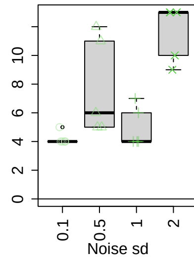
False positives
