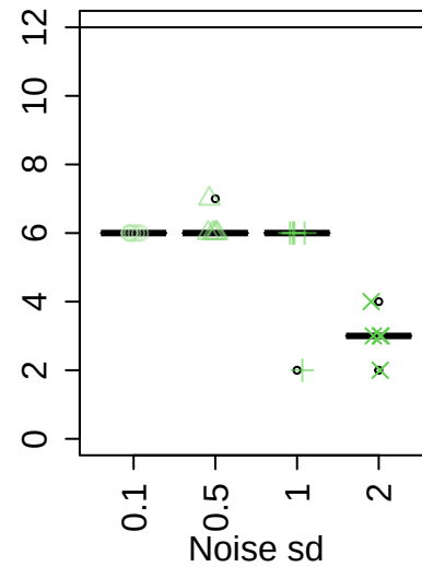
True positives
