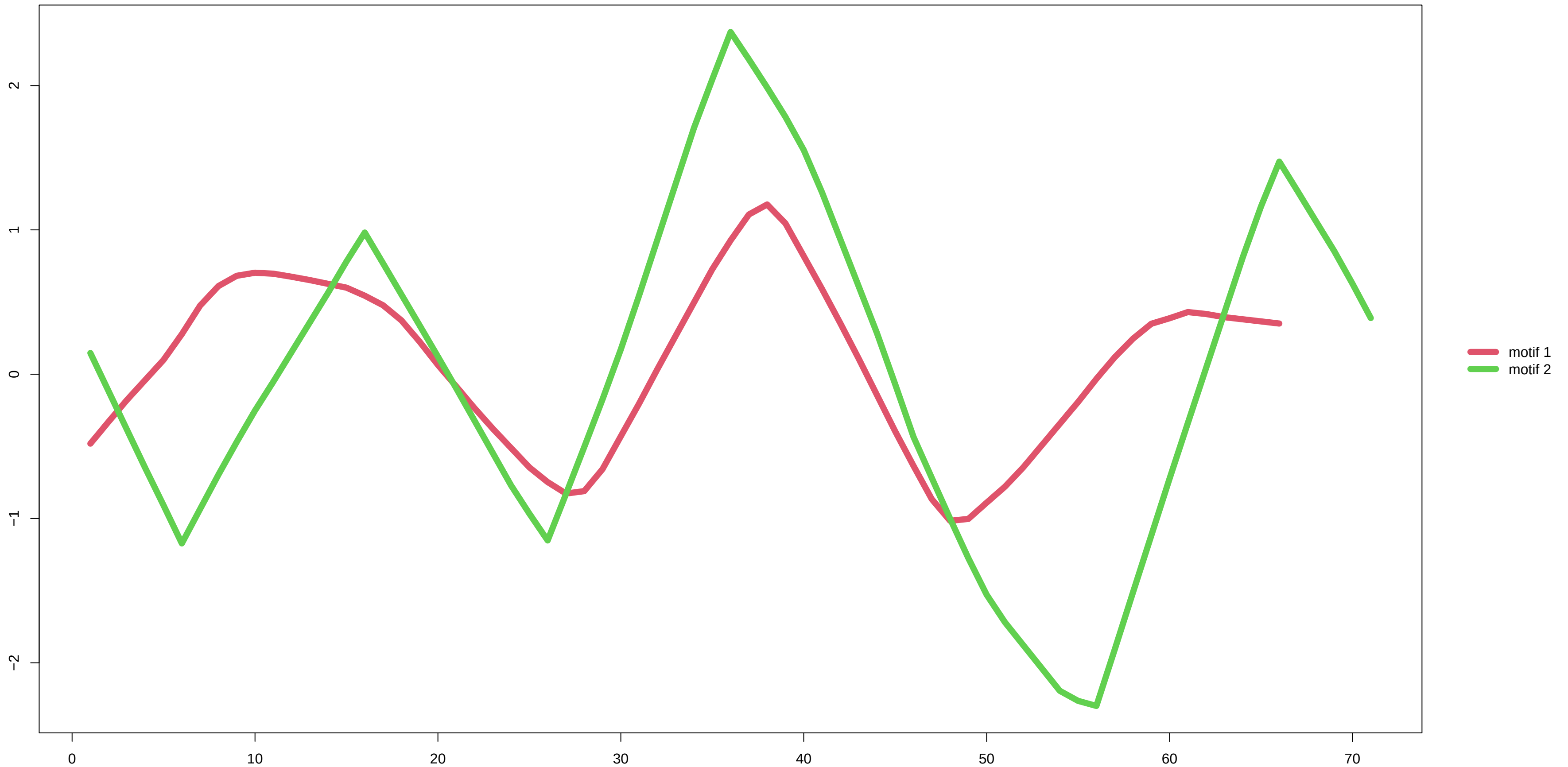
derivative
