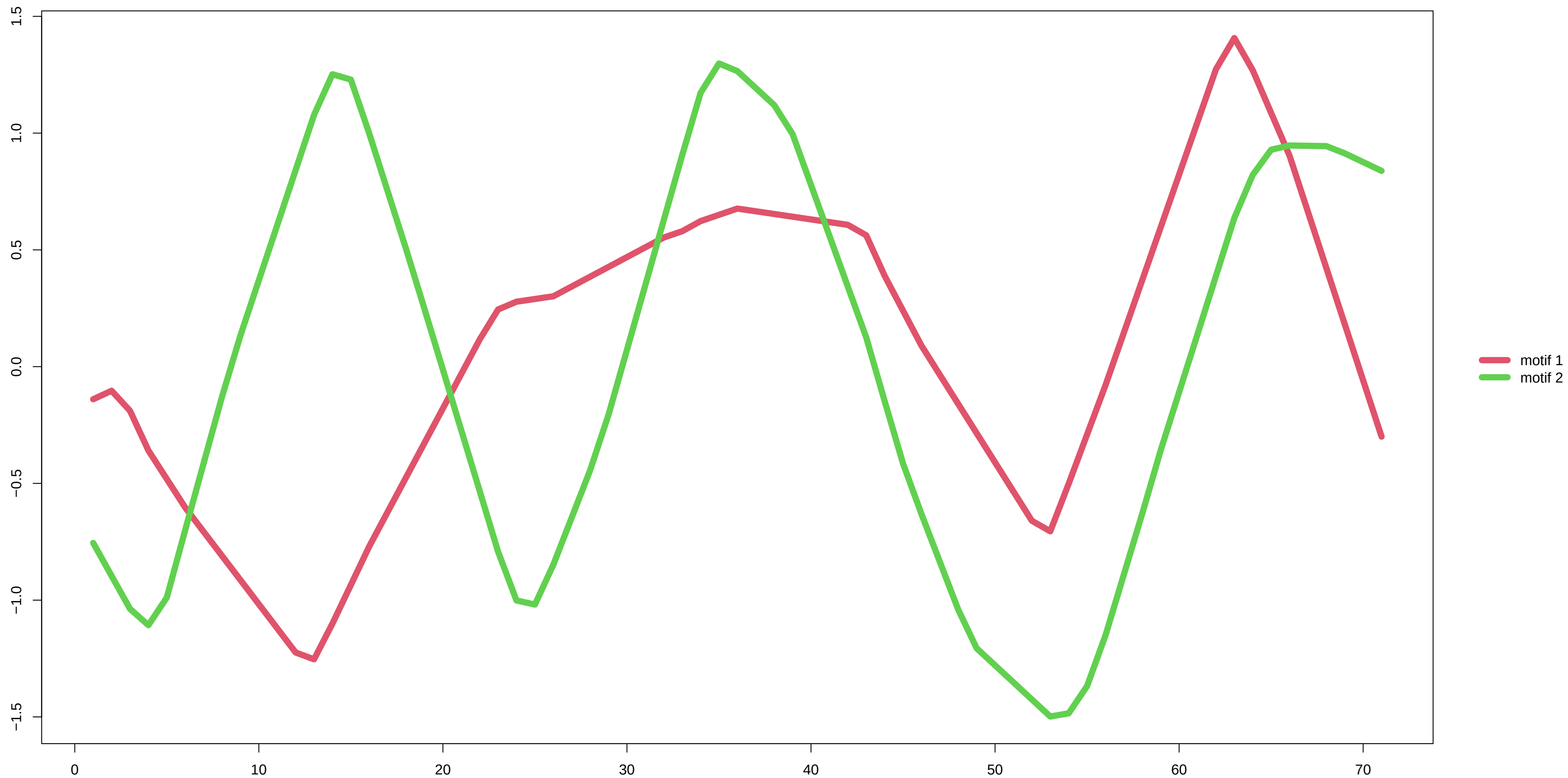
derivative
