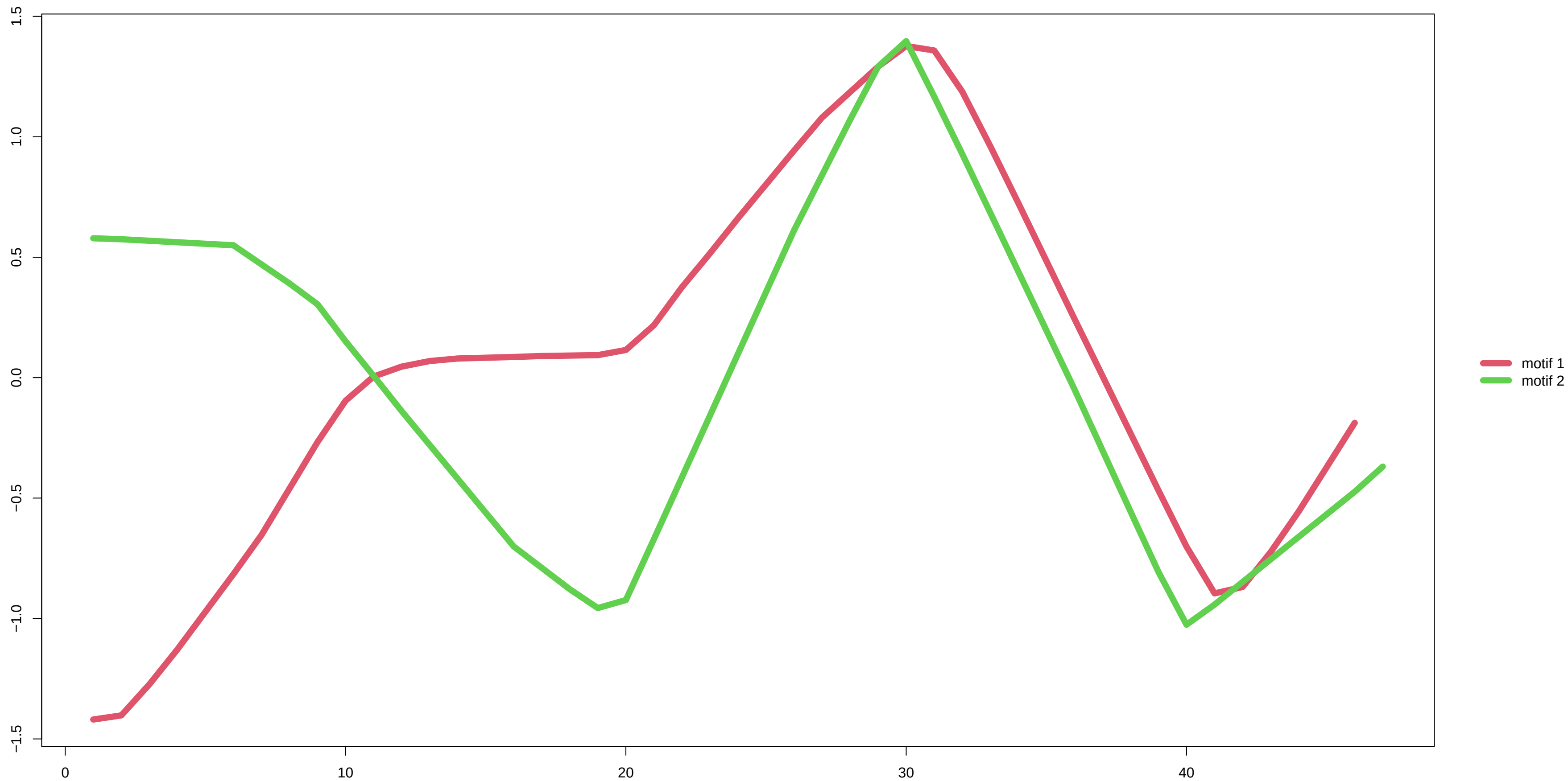
derivative
