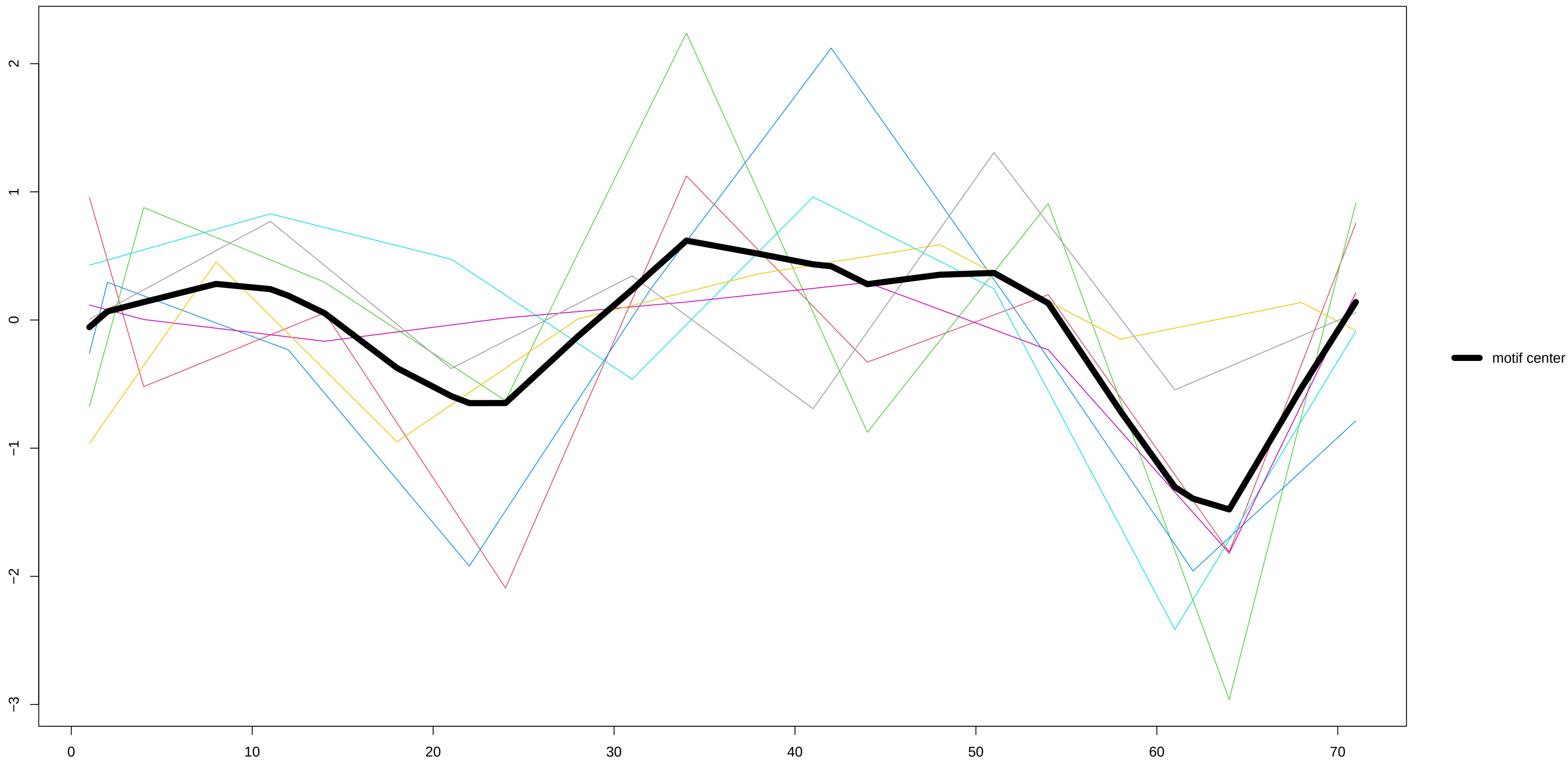
Motif 3 – derivative
