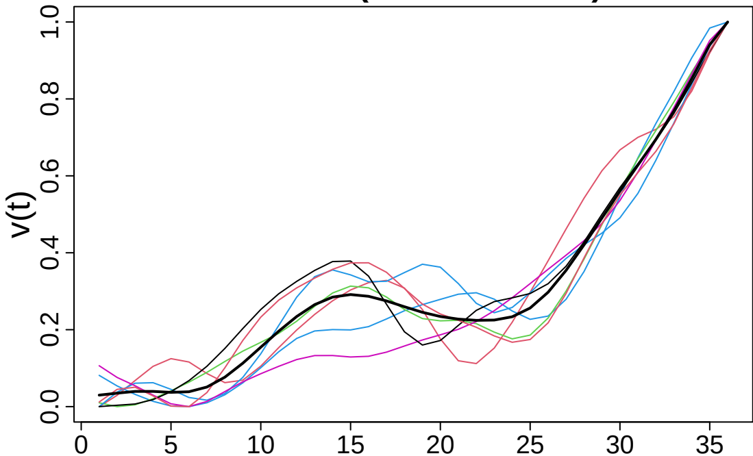
Motif 22 (7 occurrences)
