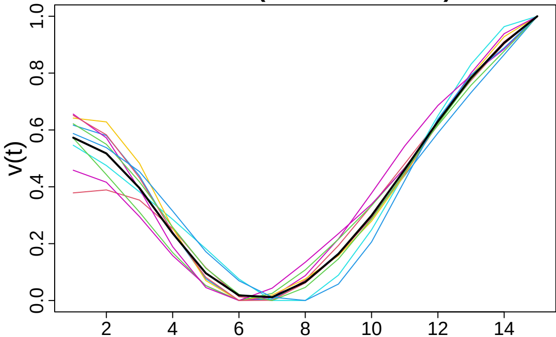
Motif 16 (10 occurrences)
