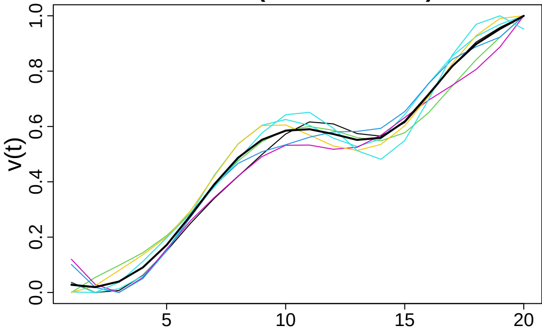
Motif 20 (7 occurrences)
