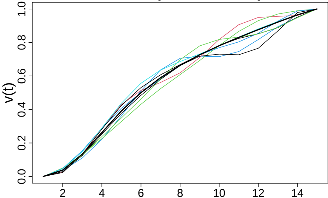
Motif 10 (8 occurrences)
