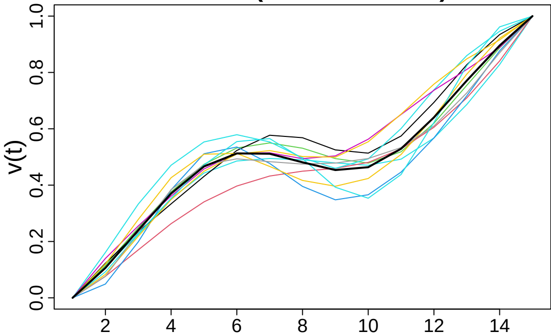
Motif 17 (11 occurrences)
