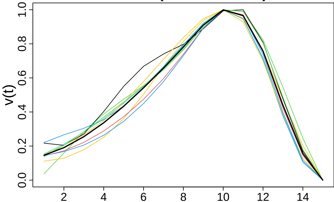
Motif 18 (9 occurrences)
