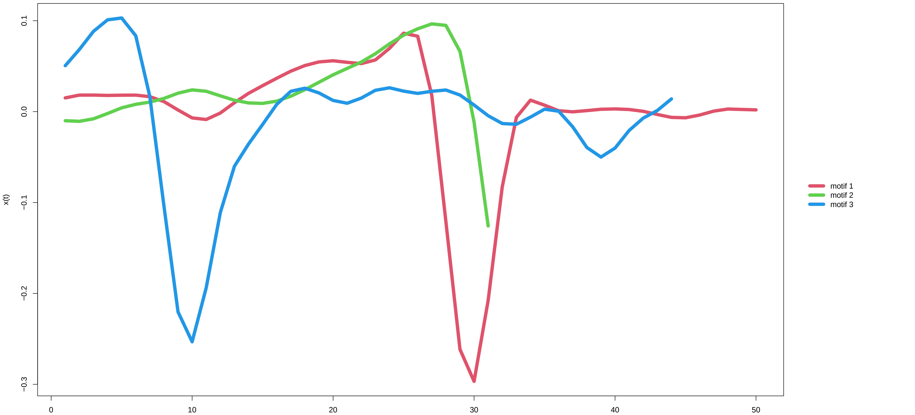
x(t) derivative
