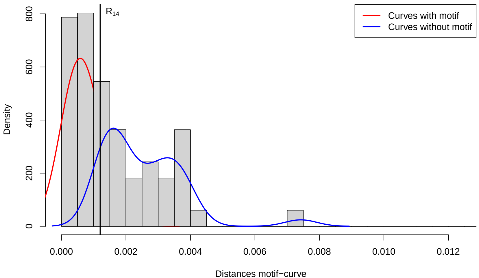
Distances motif-curve – Cluster 14
