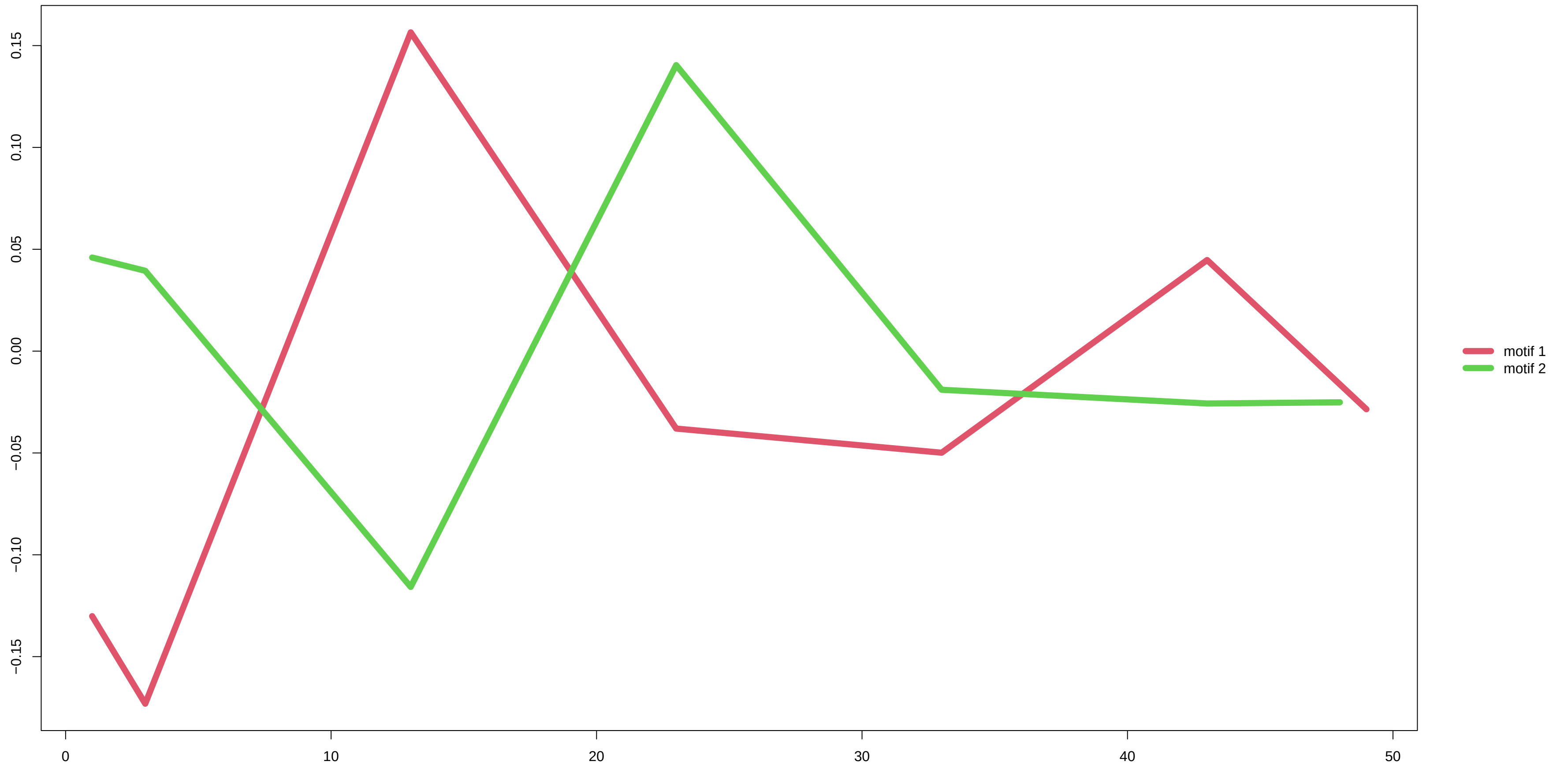
derivative
