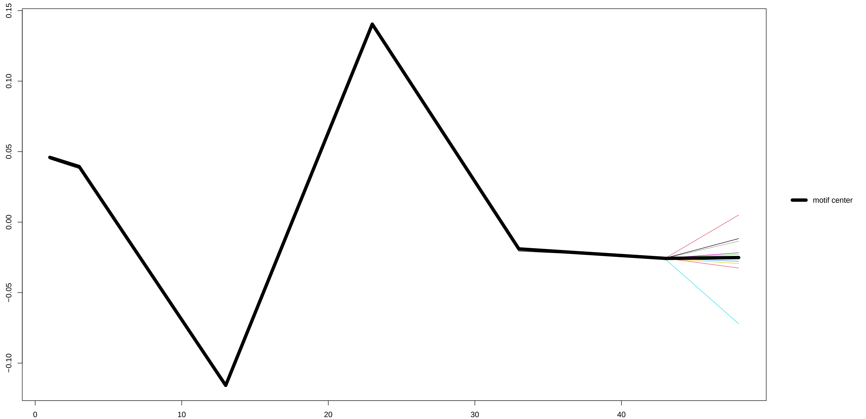
Motif 2 – derivative
