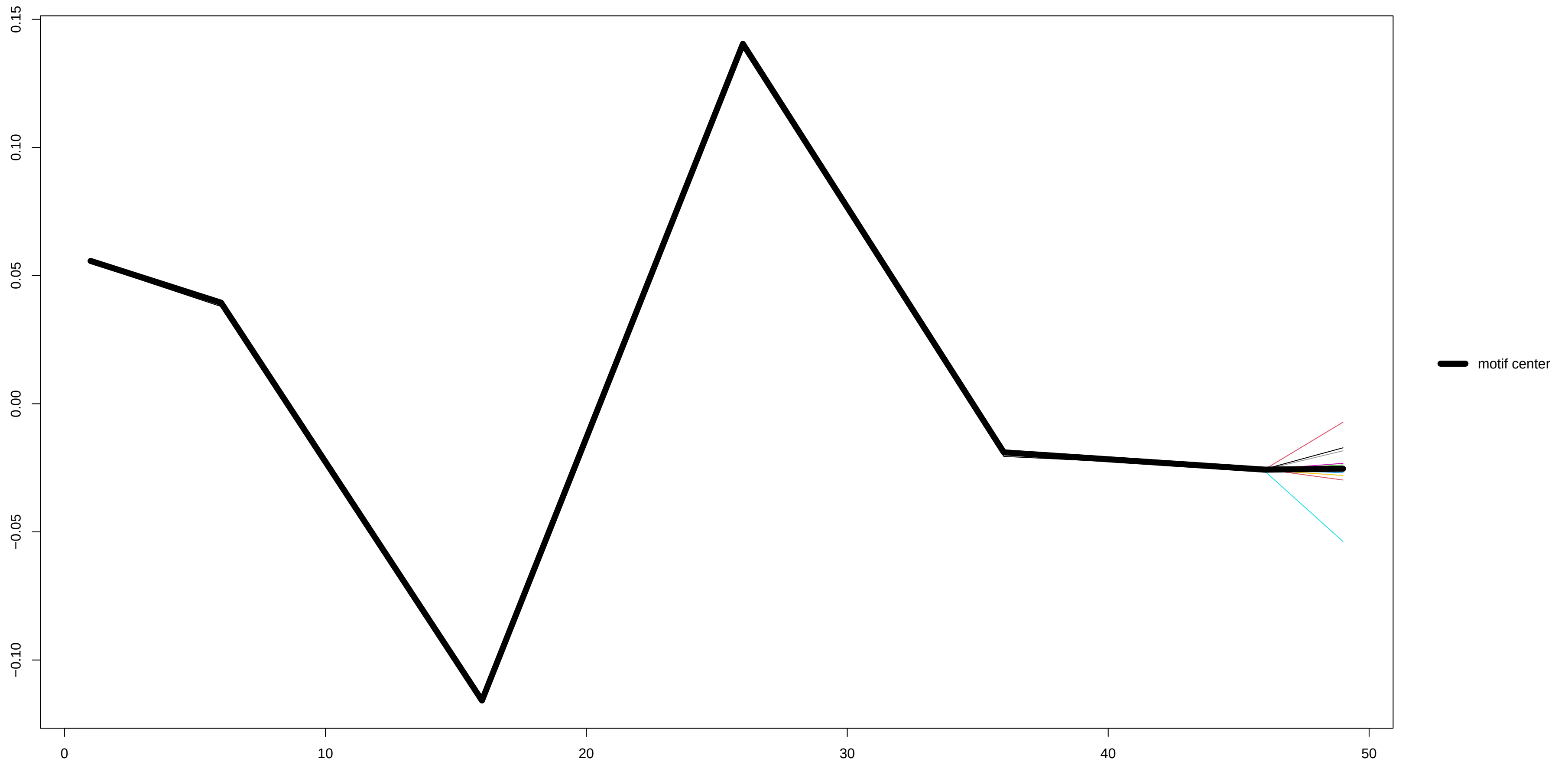
Motif 1 – derivative
