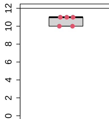
True positives
