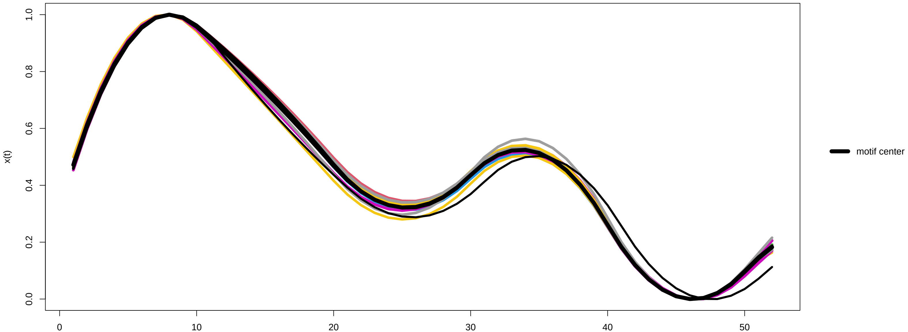
Motif 3 (11 occurrences) – x(t)
