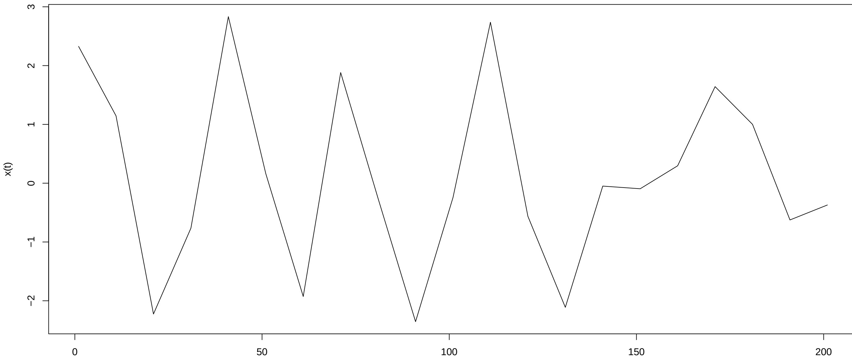
Curve 20 – x(t) derivative
