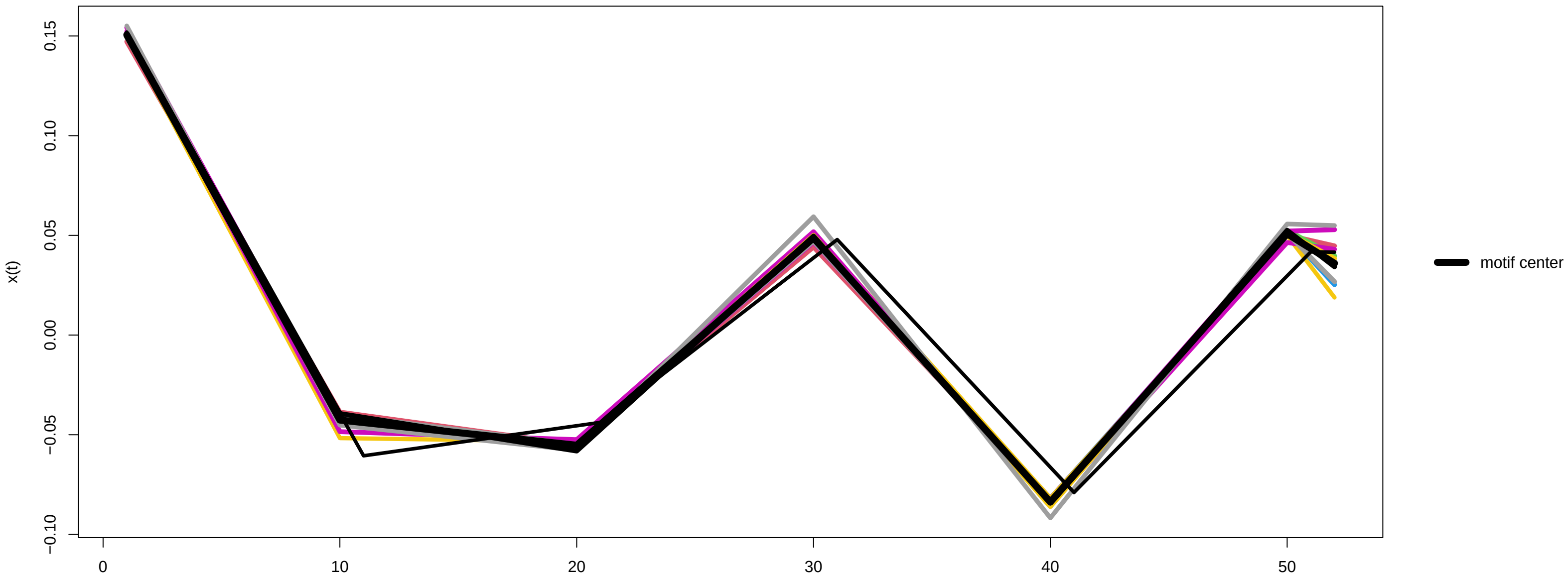
Motif 3 (11 occurrences) – x(t) derivative
