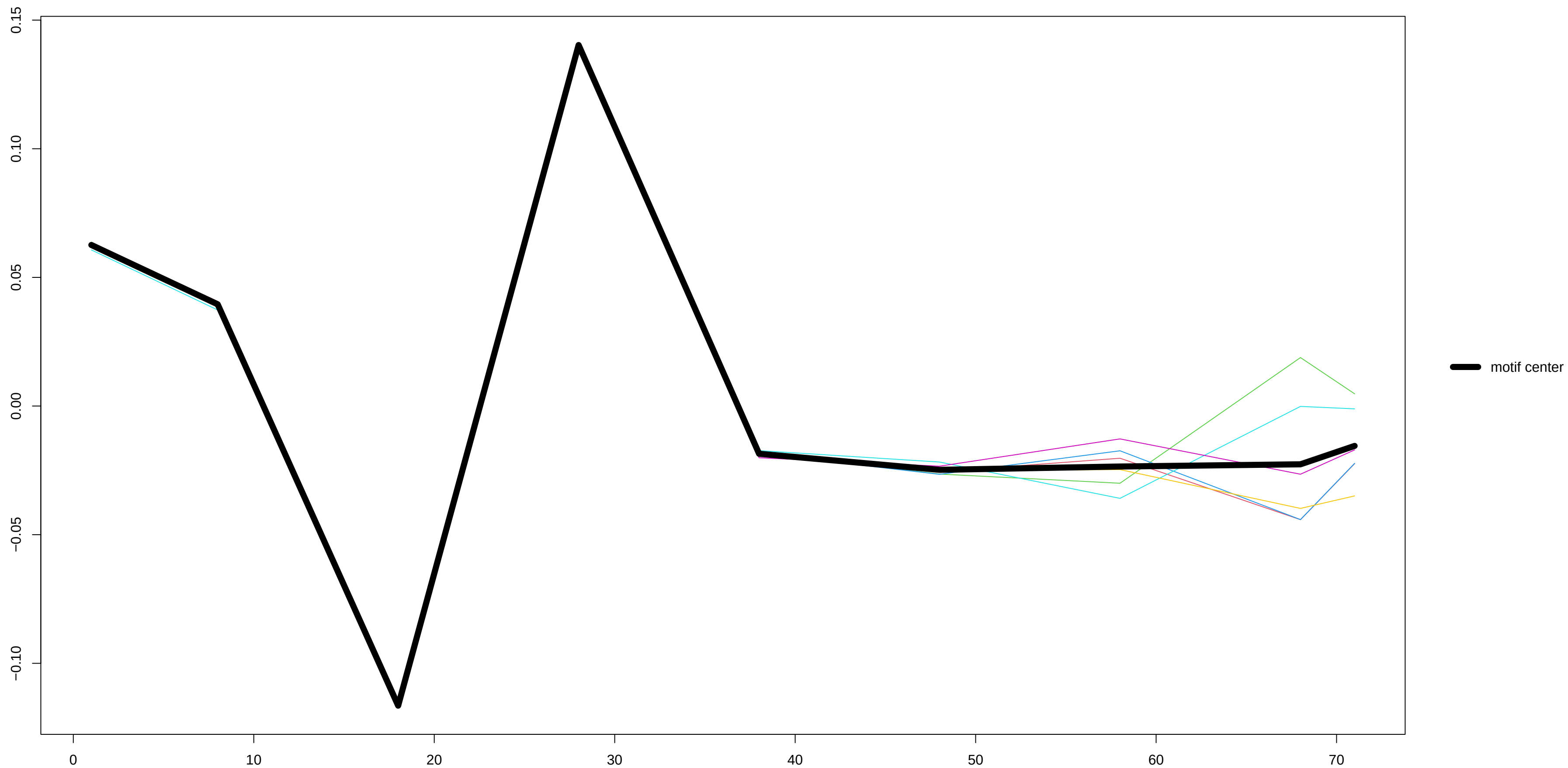
Motif 1 – derivative
