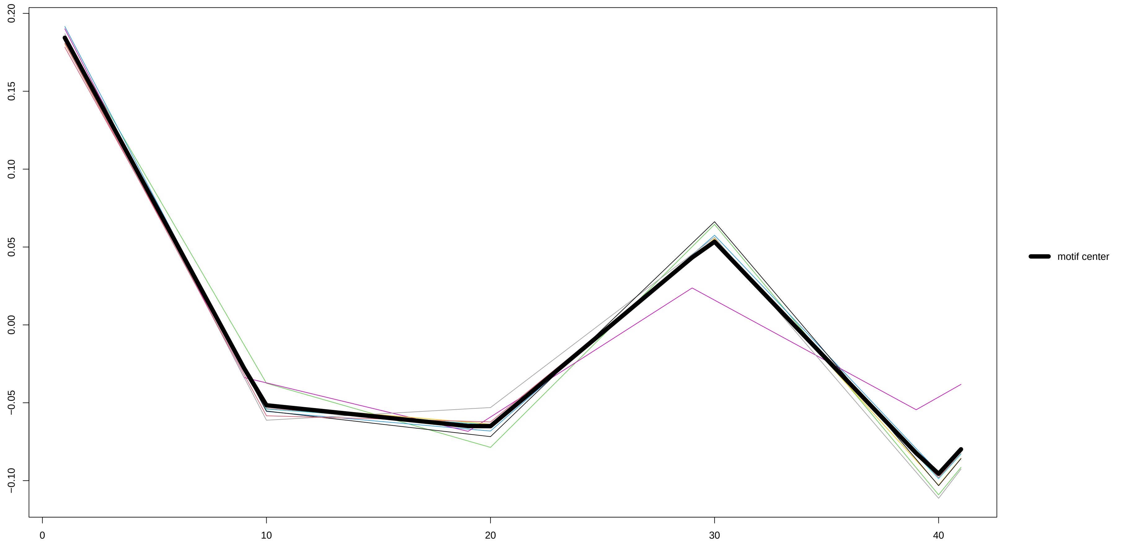
Motif 2 – derivative
