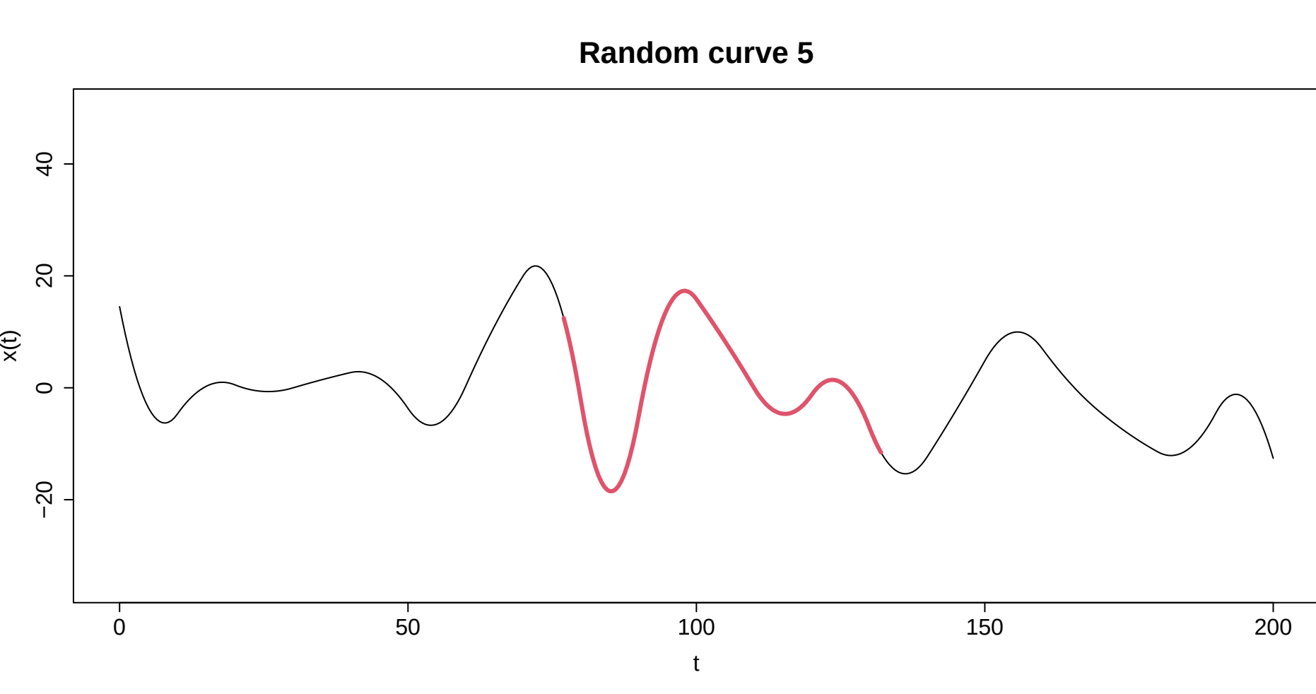
Random curve
